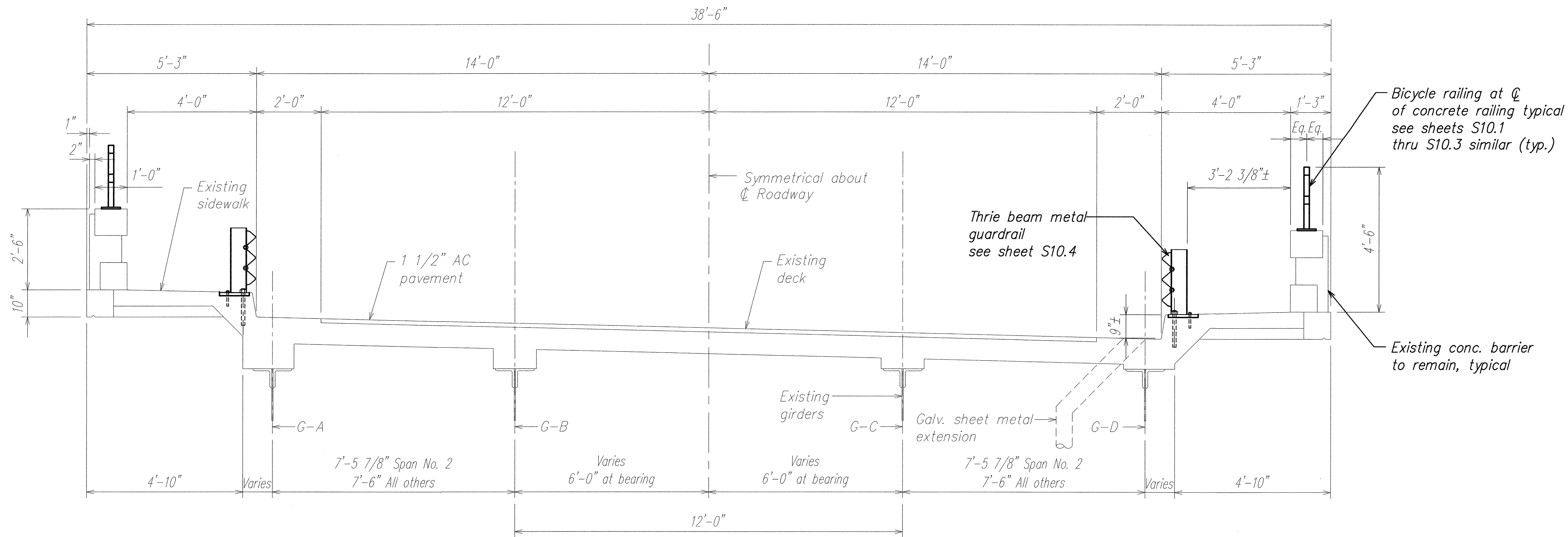
NEW DECK SECTION A SCALE: 1/2" = 1'-0" S6.3 | S6.3
