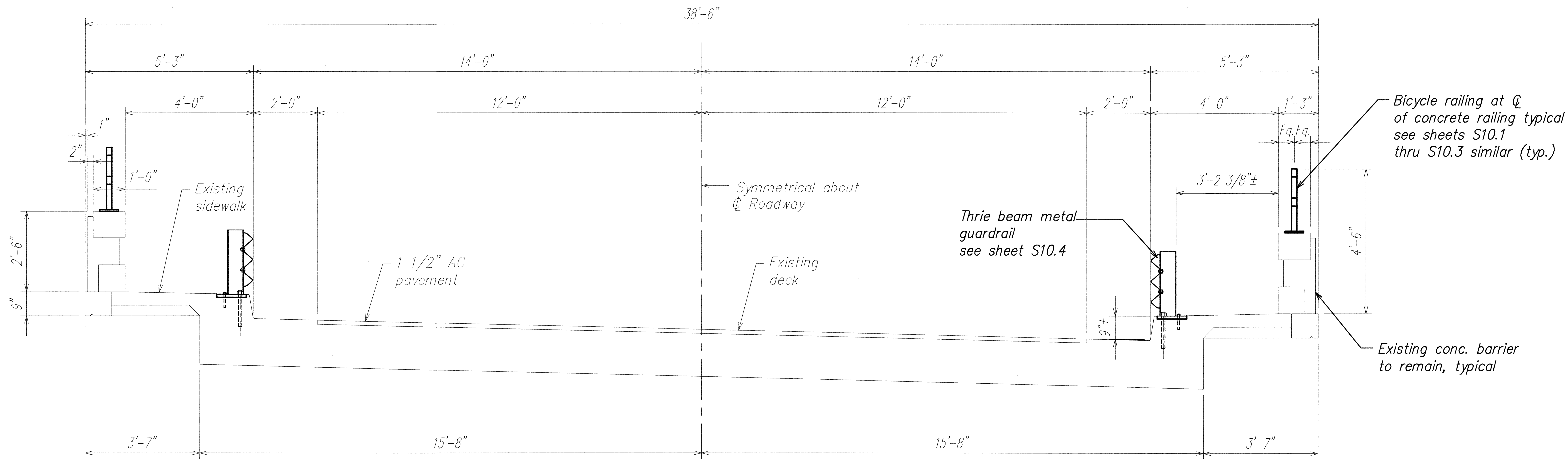
NEW DECK SECTION A SCALE: 1/2" = 1'-0" S6.3 | S6.3
