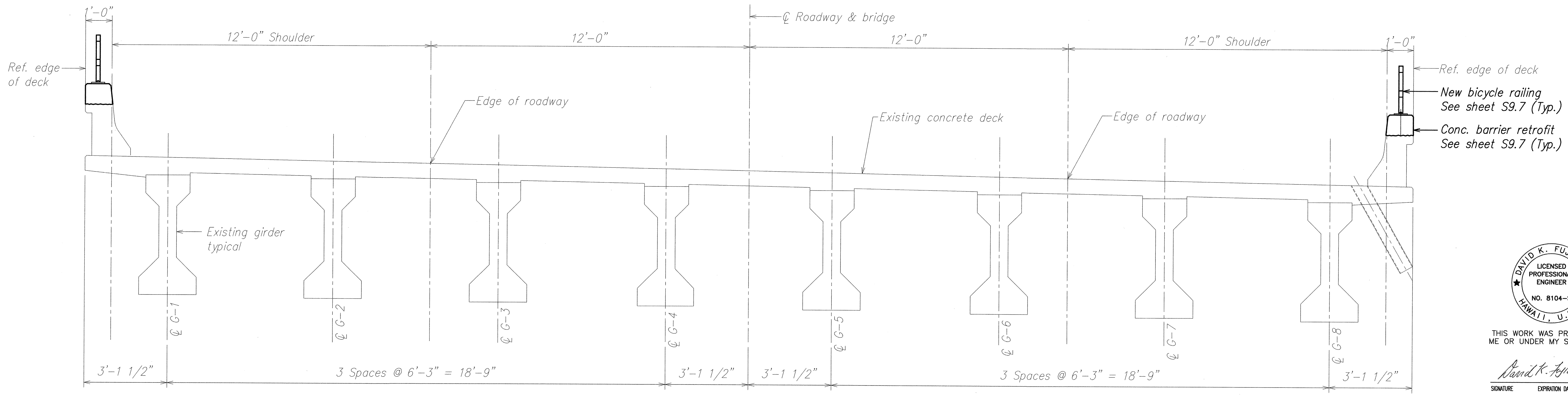
NEW NORMAL DECK SECTION A SCALE: 1/2" = 1'-0"
