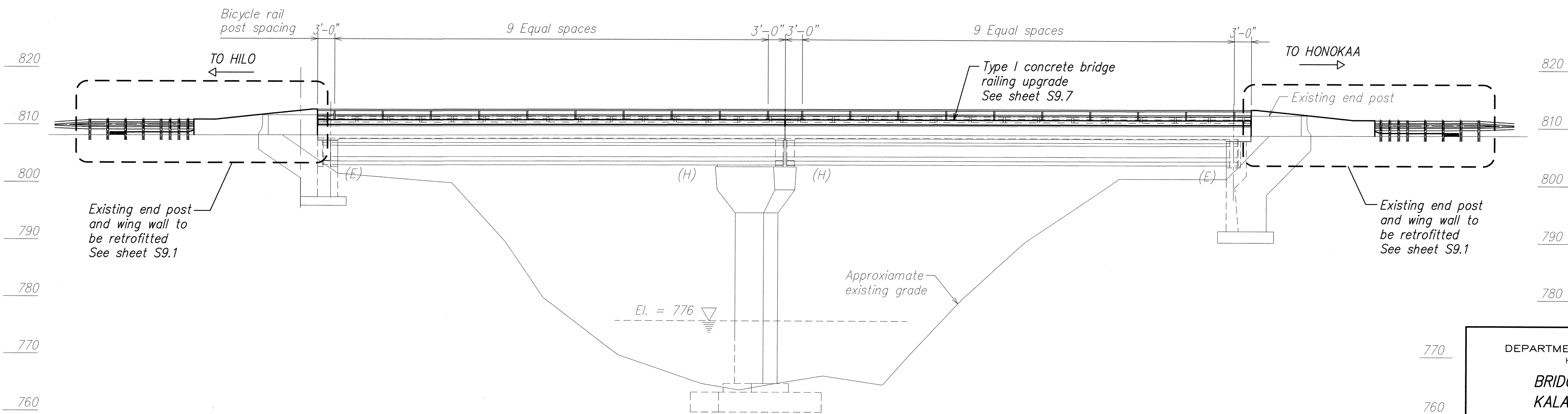
BRIDGE - ELEVATION B SCALE: 1" = 10'-0" S5.3 S5.3
