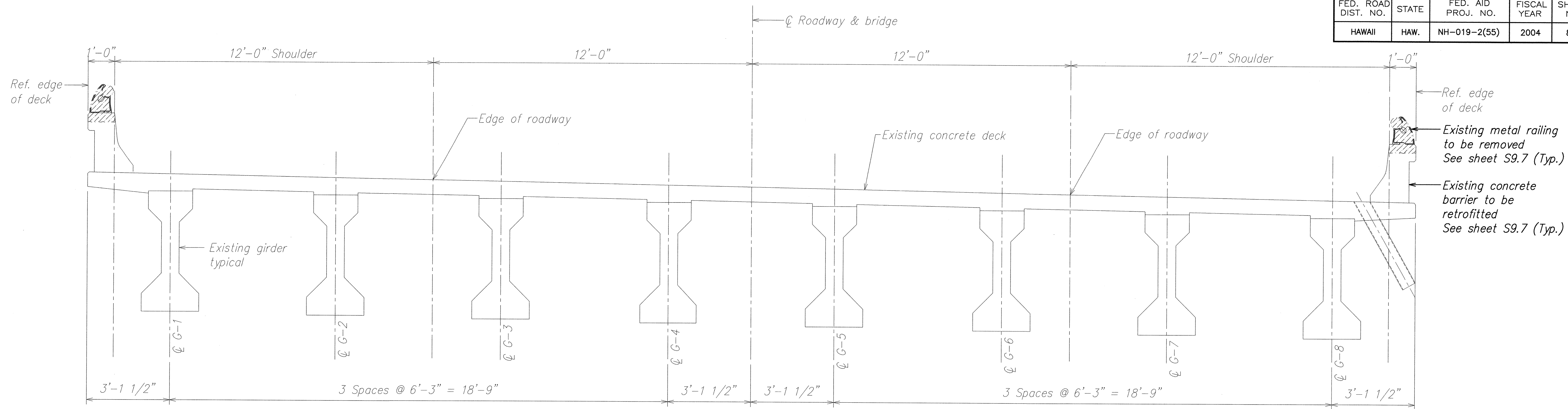
EXISTING NORMAL DECK SECTION A SCALE: 1/2" = 1'-0"
