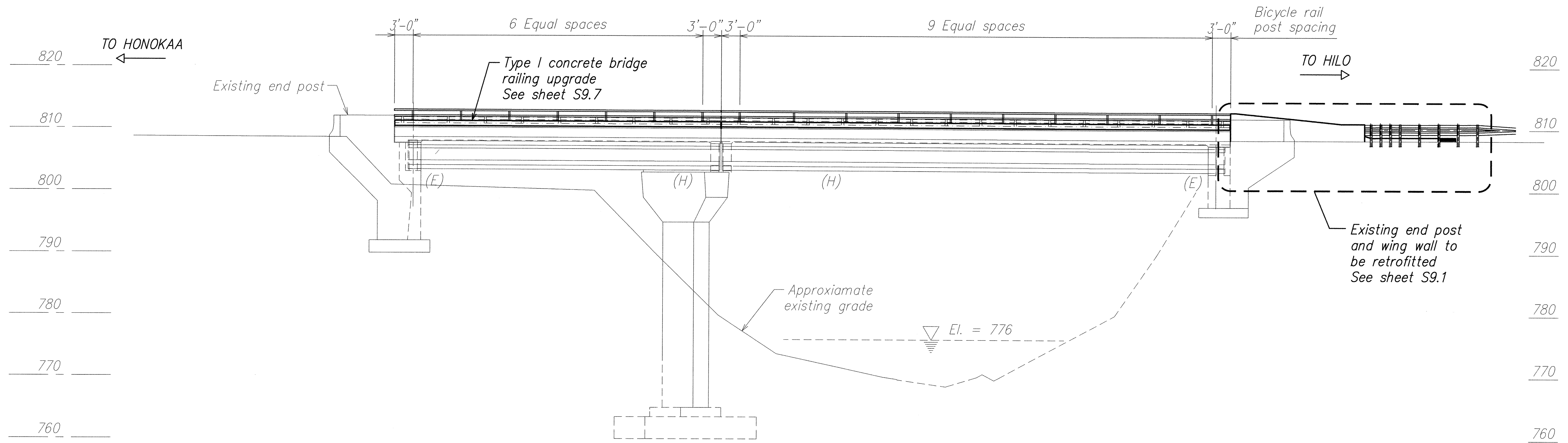
BRIDGE - ELEVATION A SCALE: 1" = 10'-0" S5.3 S5.3
