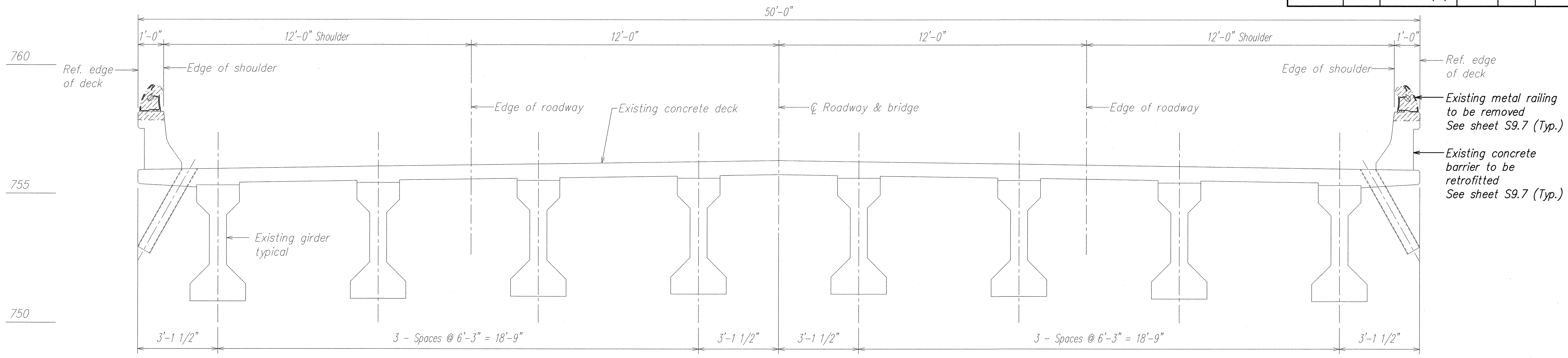
EXISTING NORMAL DECK SECTION A SCALE: 1/2" = 1'-0" S2.2 S2.2
