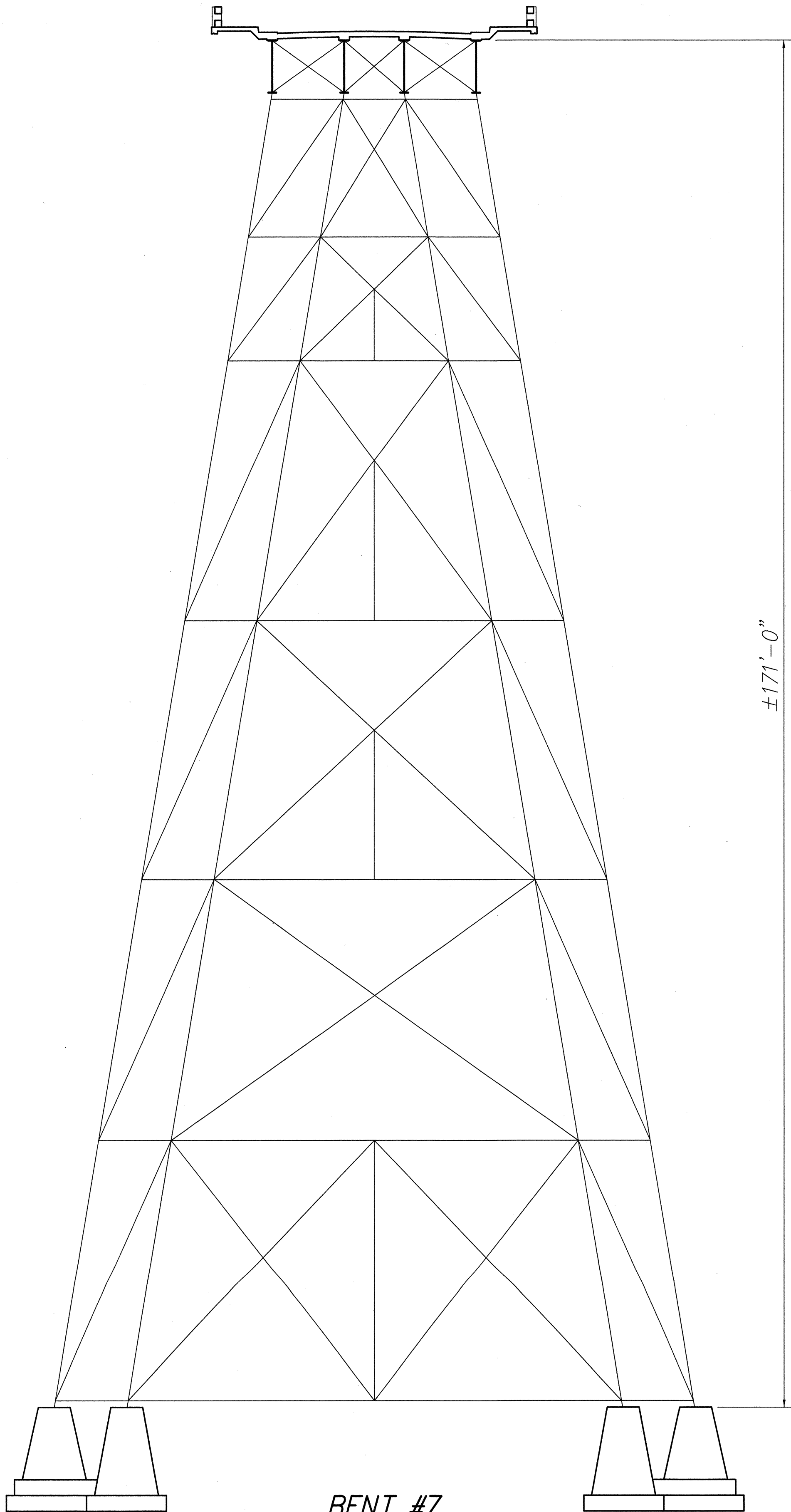
BENT #7
