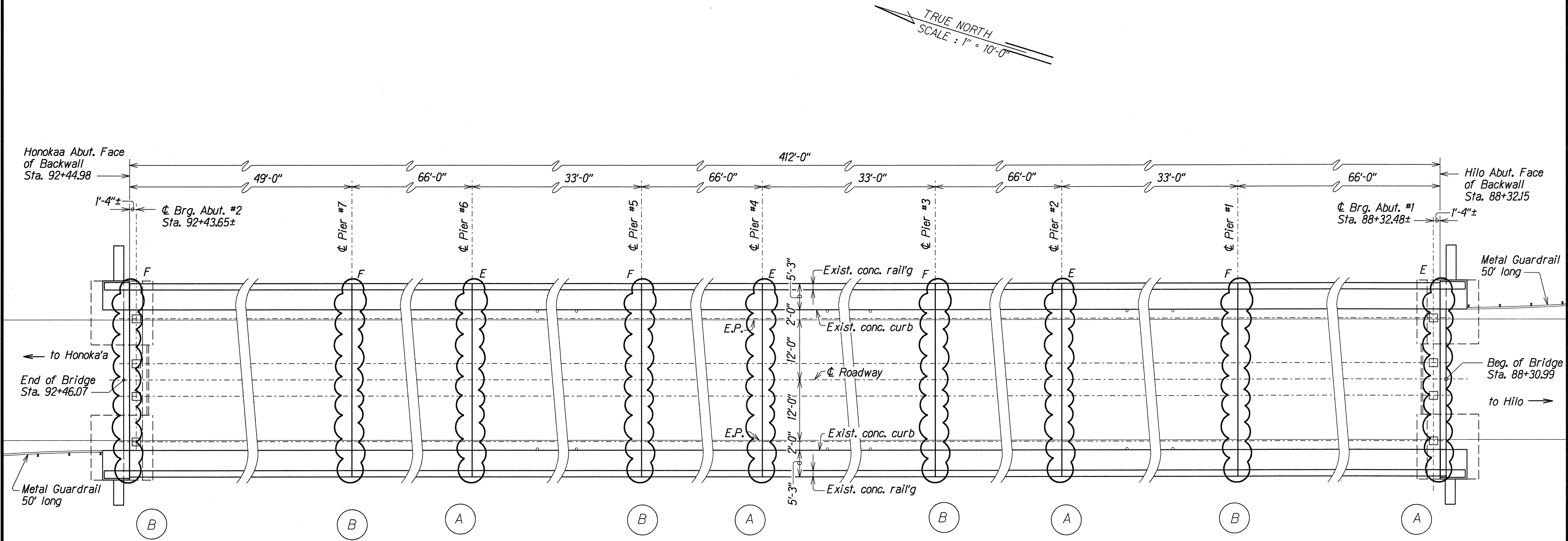
LAYOUT PLAN--KAPUE BRIDGE Scale: 1" = 10'-0"
