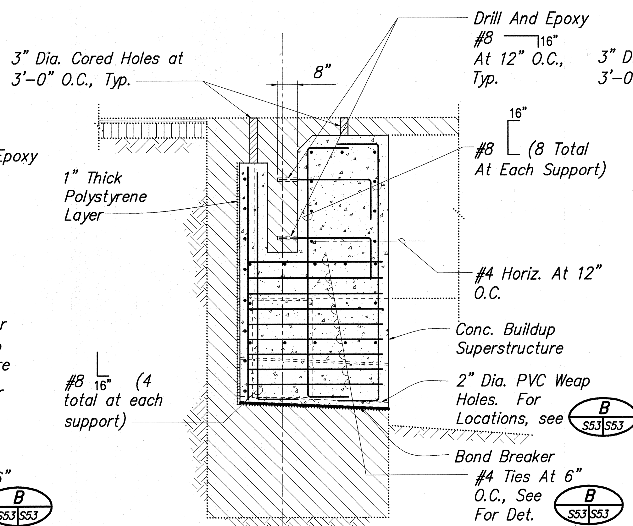
DETAIL 2 SCALE: 1/2"=1'-0" S53/S56
