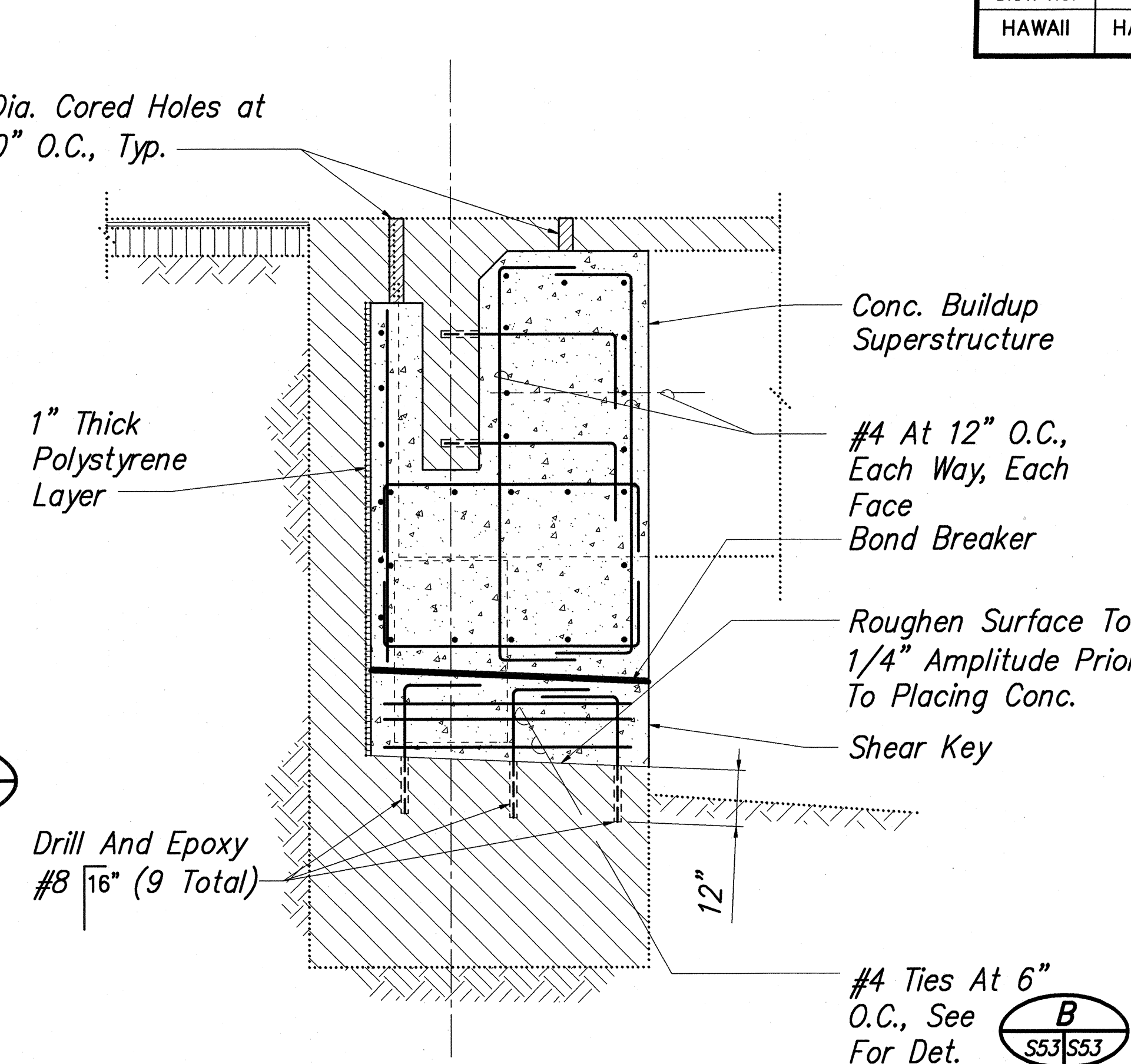
DETAIL 3 SCALE: 1/2"=1'-0" S53/S56
