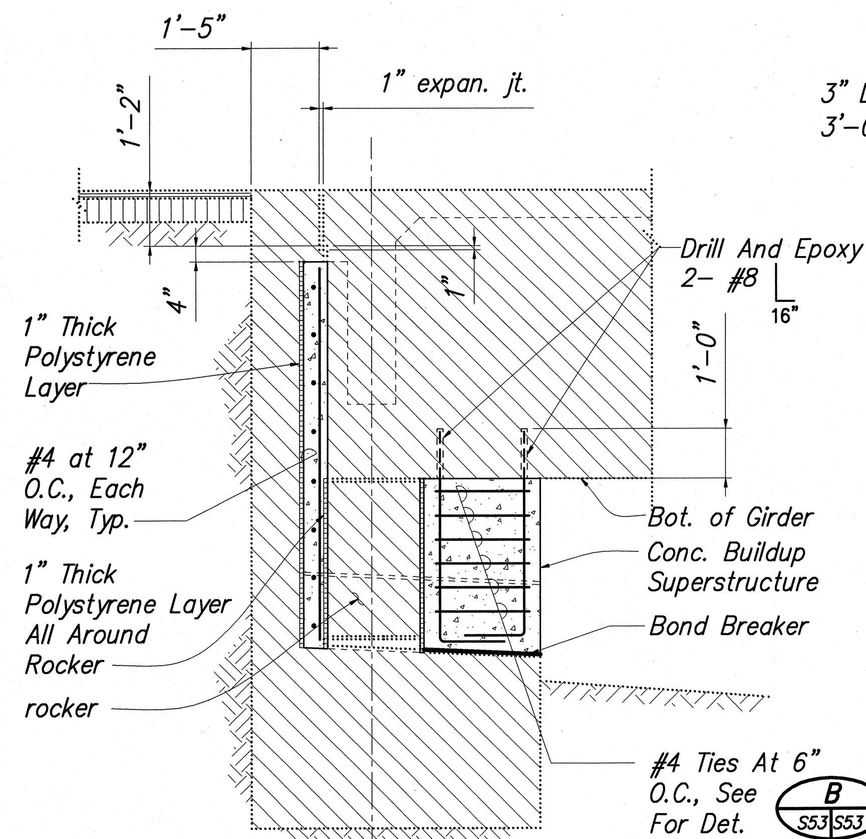
DETAIL 1 SCALE: 1/2"=1'-0" S53/S56
