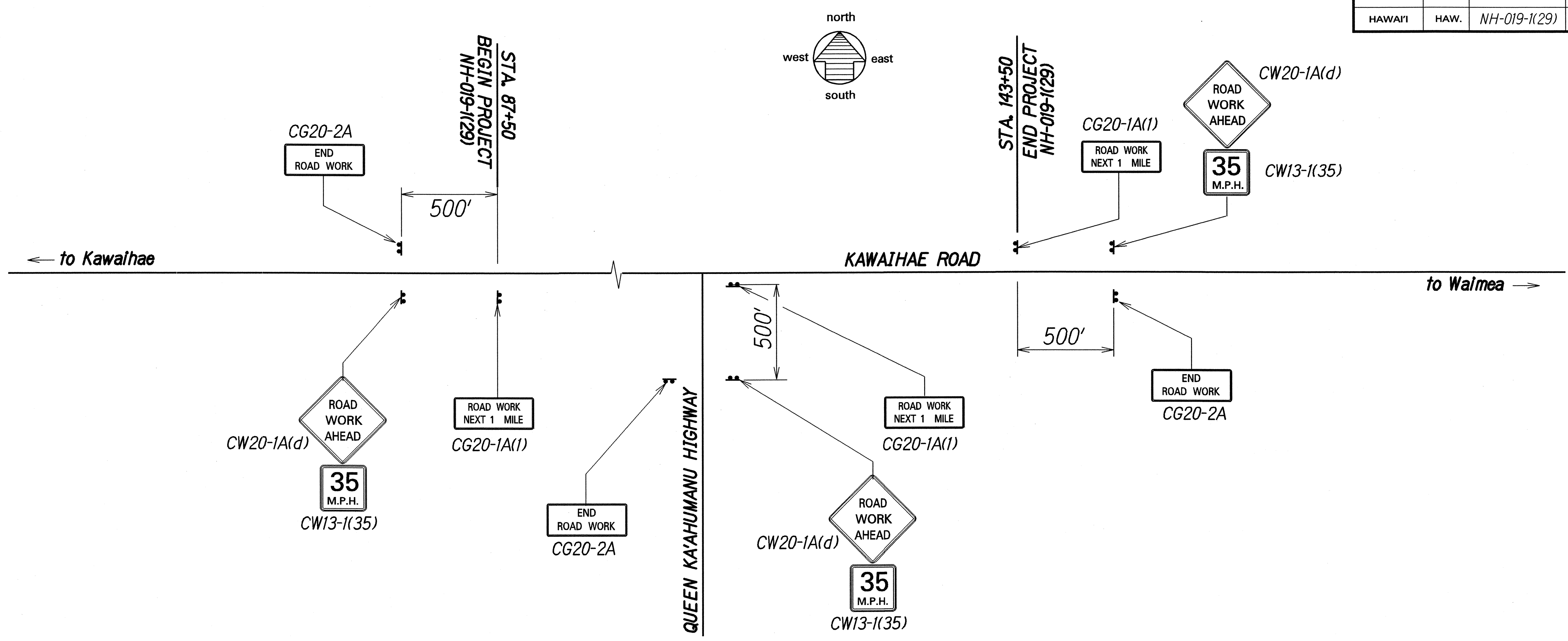
CONSTRUCTION SIGN PLAN Not To Scale
