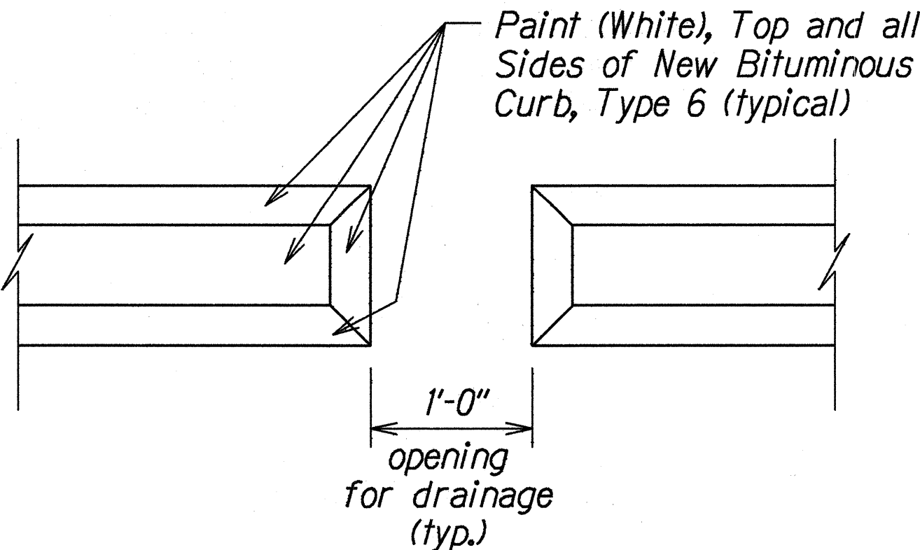
BITUMINOUS CURB
