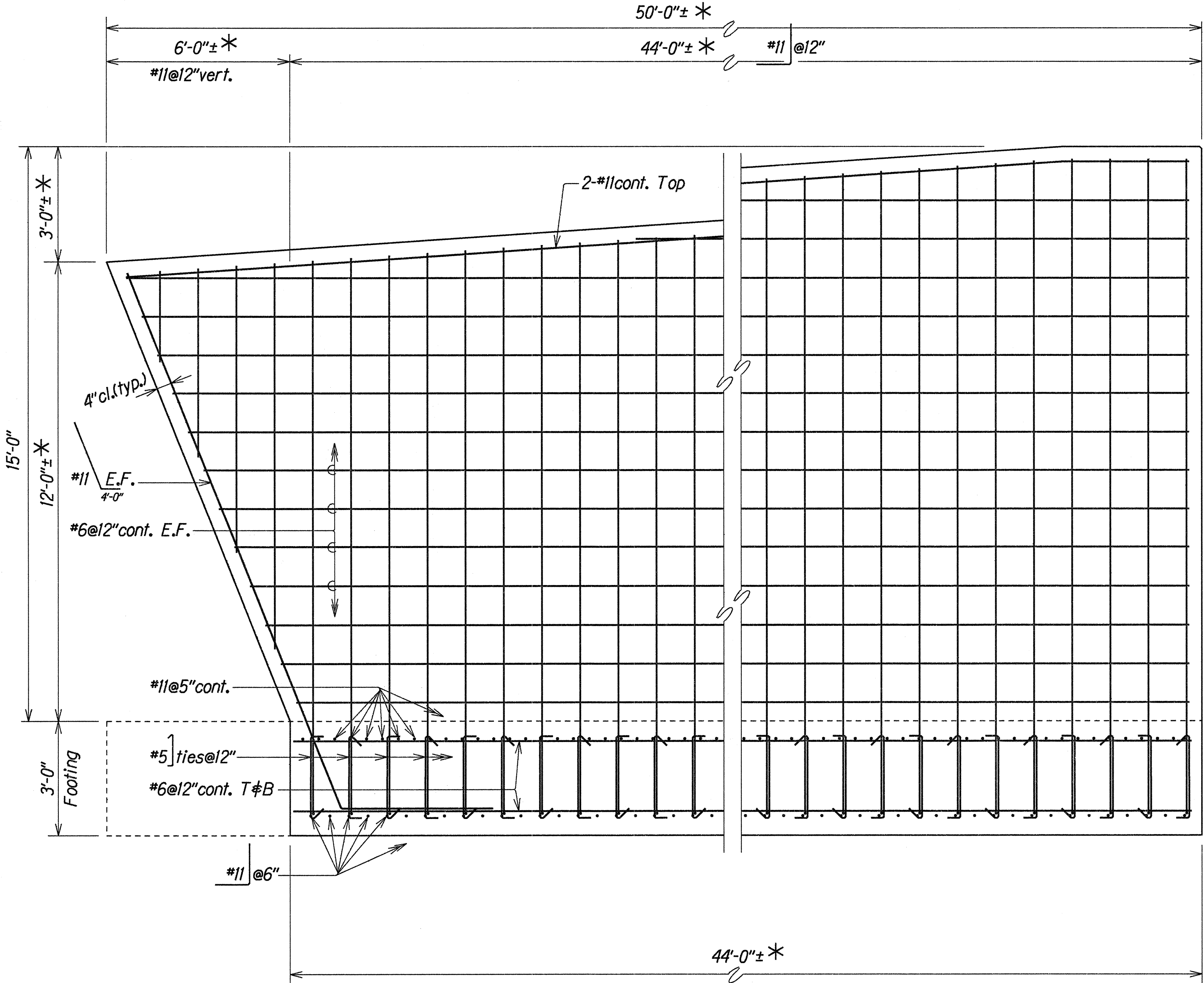
FRONT FACE
