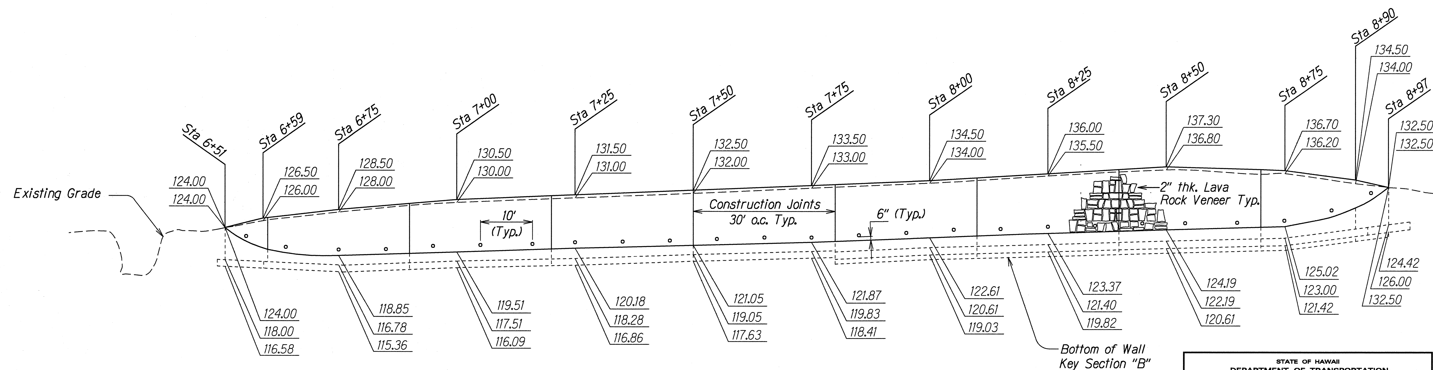
RETAINING WALL ELEVATION
