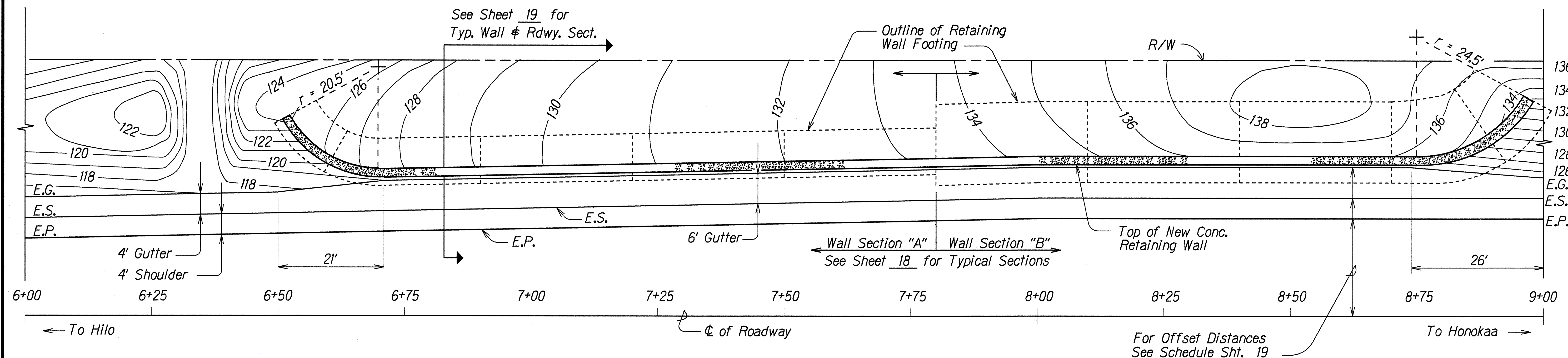
RETAINING WALL PLAN
