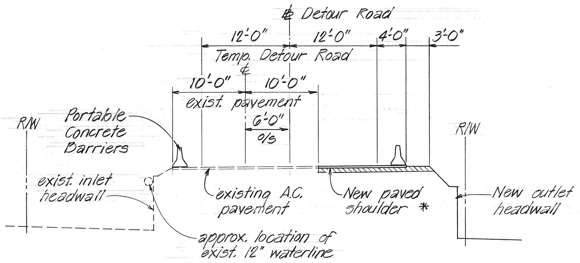
TYPICAL SECTION - DETOUR ROAD @ STA. 109+70 Scale: 1/8" = 1'-0"
