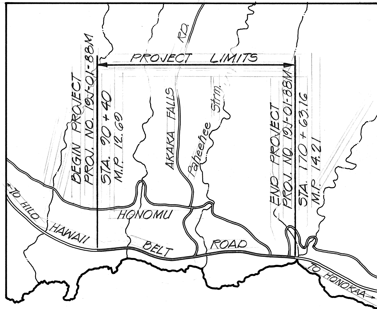
GENERAL LOCATION PLAN Scale: 1" = 2000'
