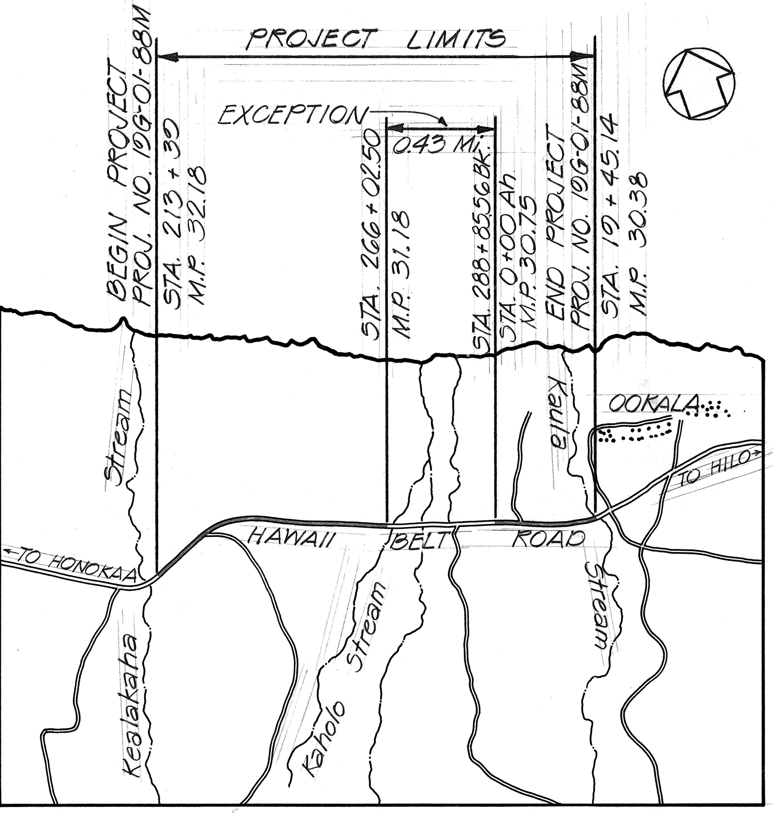
GENERAL LOCATION PLAN Scale: 1" = 2000'
