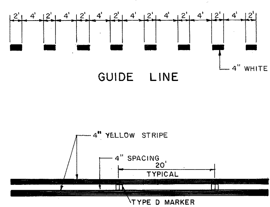
DOUBLE YELLOW CENTERLINE (COUNTY STREET)
