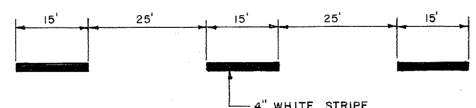
SINGLE DASHED LANE LINE (COUNTY STREET)
