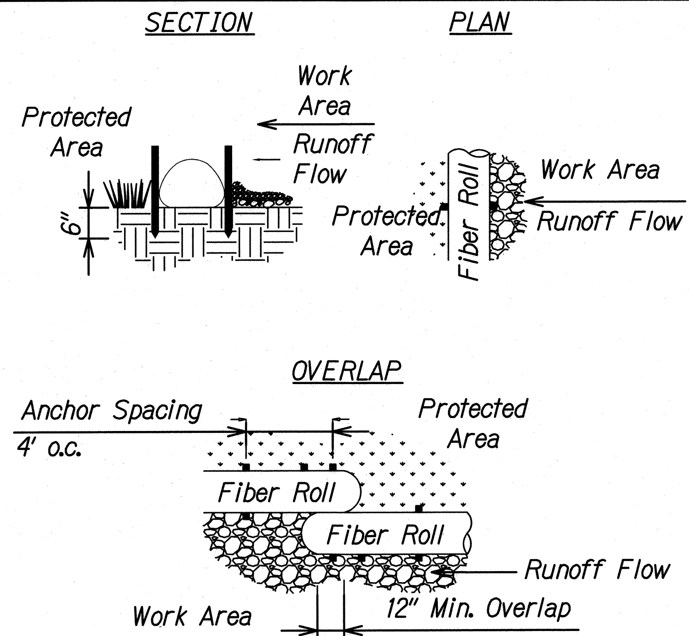
BMP DETAIL-FIBER ROLL FILTER SEDIMENT CONTROL Not To Scale
