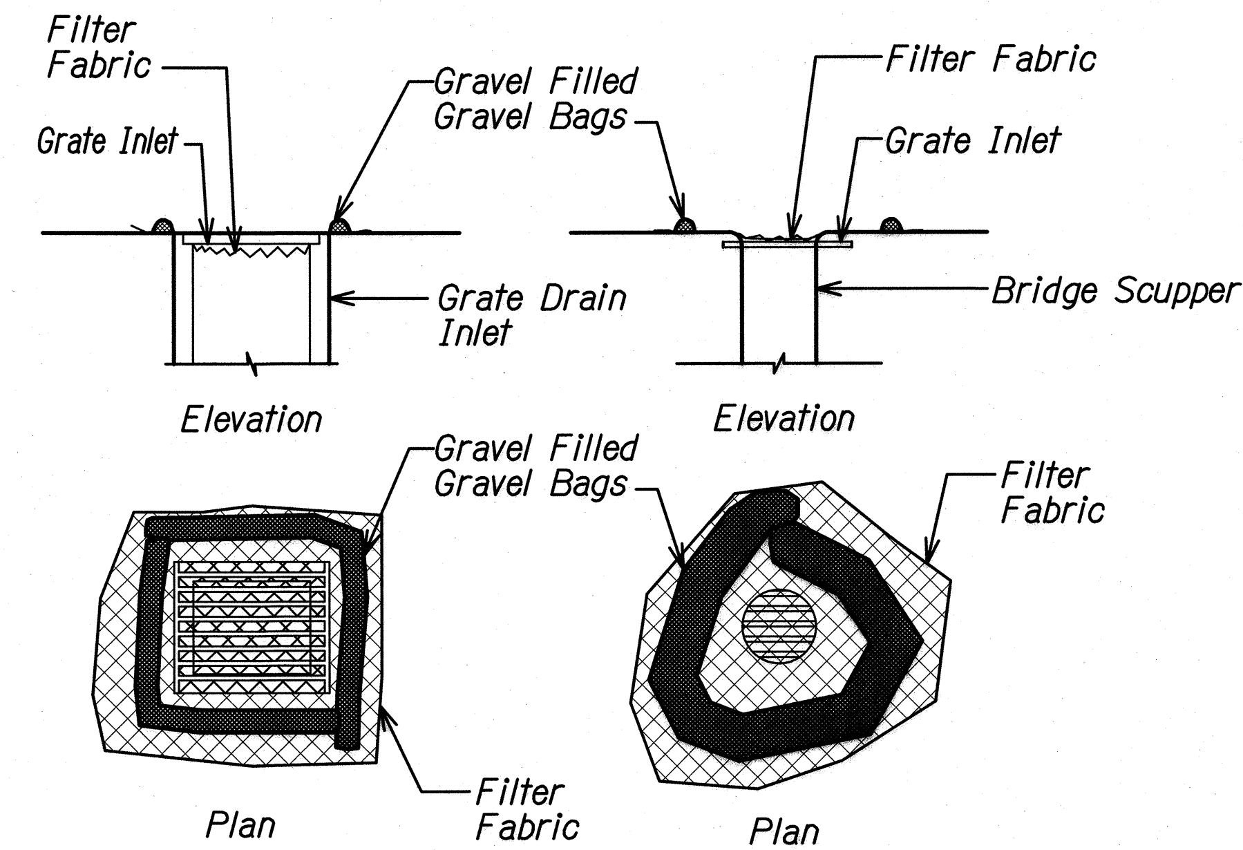
SEDIMENT BARRIER FOR DRAIN INLET Not to Scale
