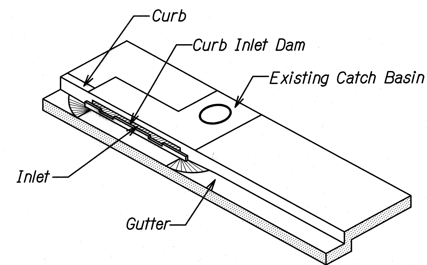
BMP DETAIL-SEDIMENT CONTROL FOR CATCH BASIN Not To Scale
