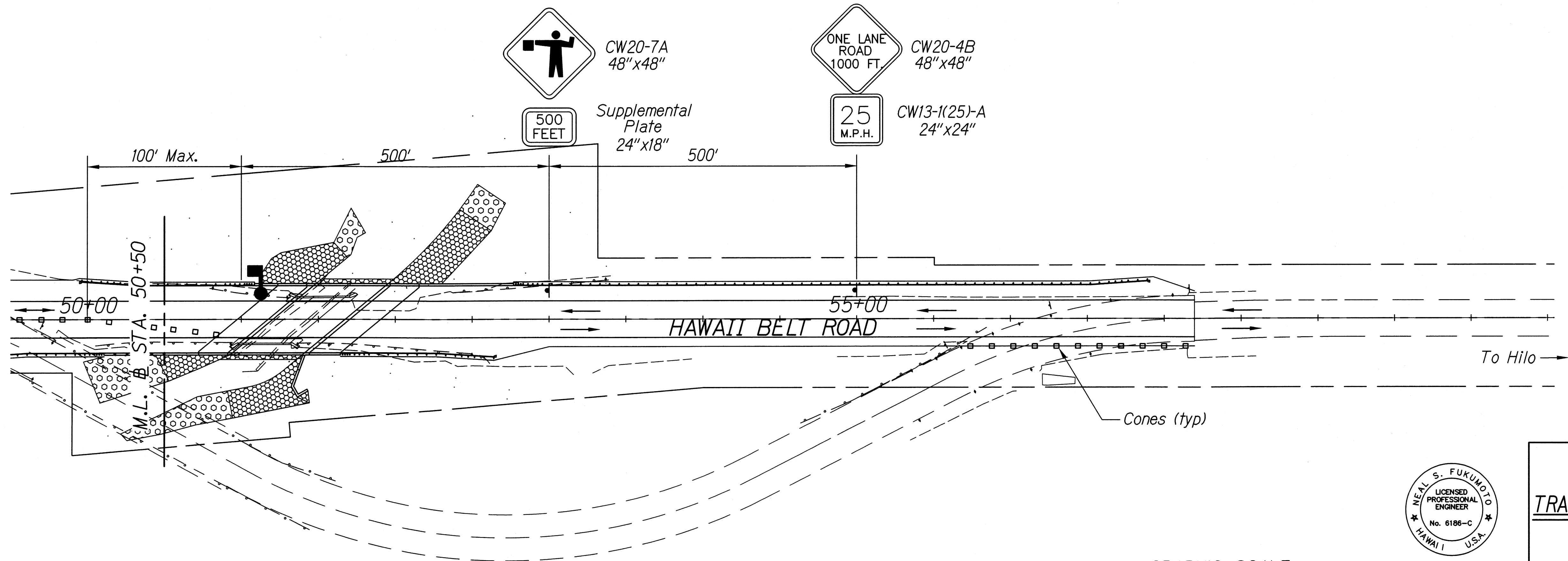
TRAFFIC CONTROL PLAN SCALE: 1"=40'
