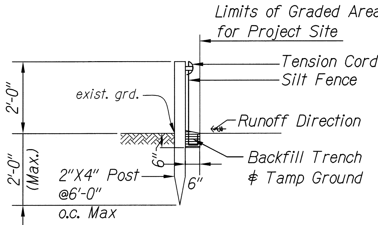
(For Overland Flow Condition) SILT FENCE DETAIL Scale: None
