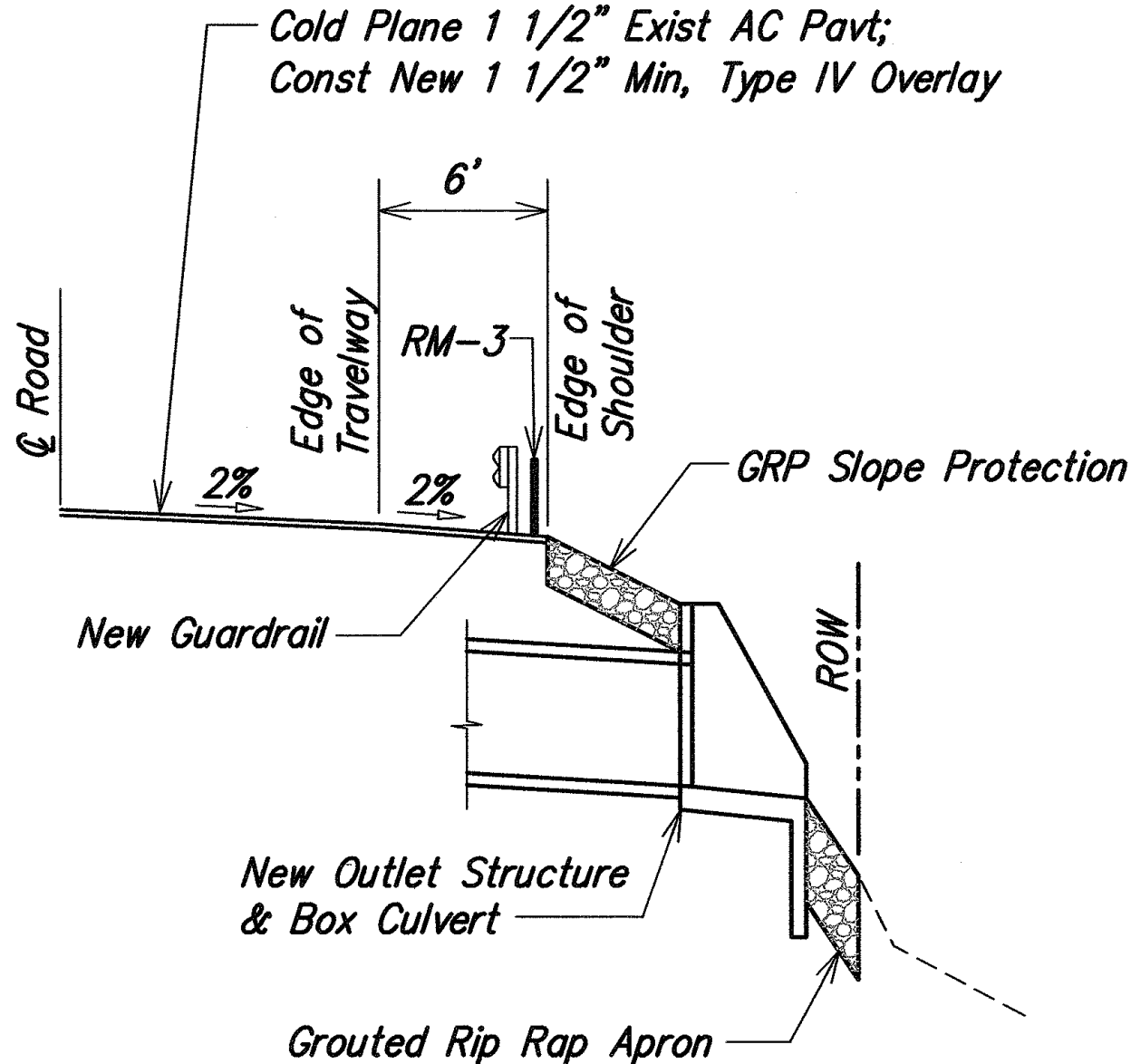
PARTIAL SECTION THRU OUTLET Not to Scale
