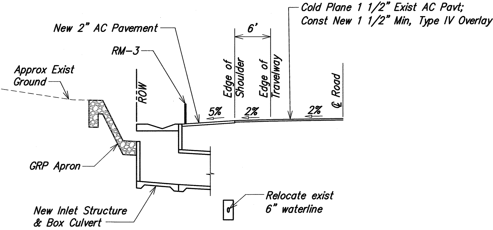
PARTIAL SECTION THRU INLET Not to Scale
