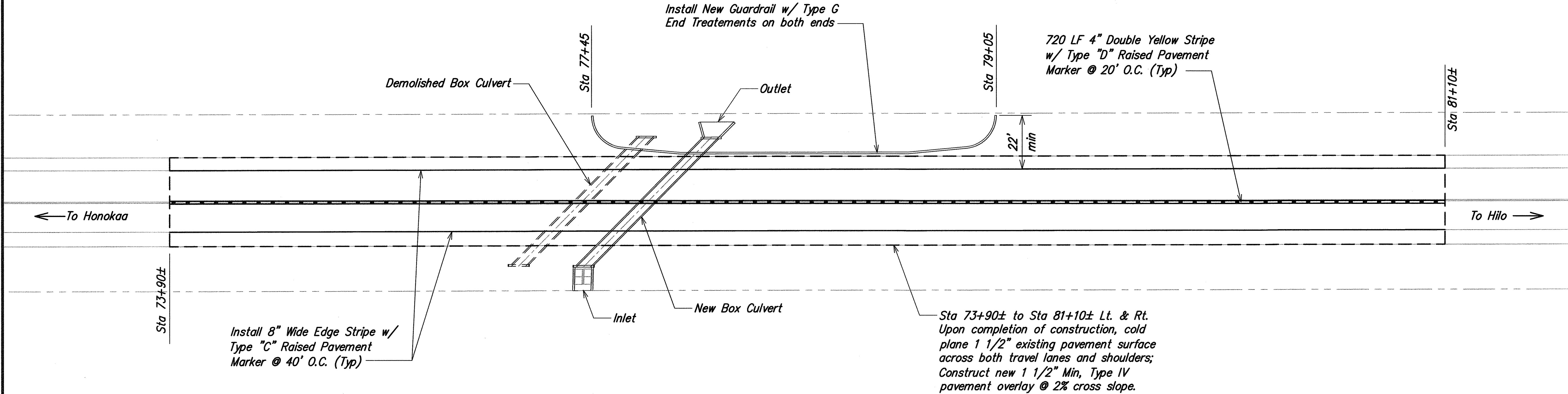
PAVING & MARKING PLAN - MP 19.36 Not to Scale
