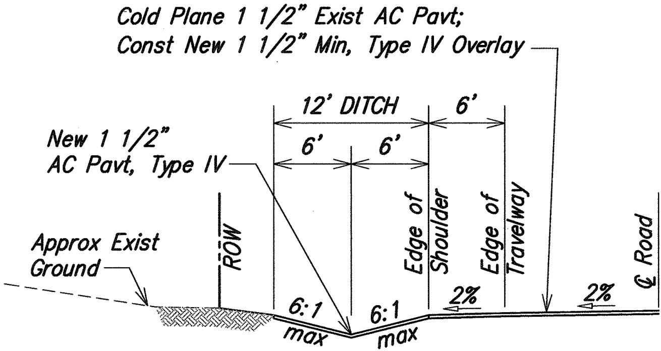
TYPICAL SECTION THRU DITCH Not to Scale
