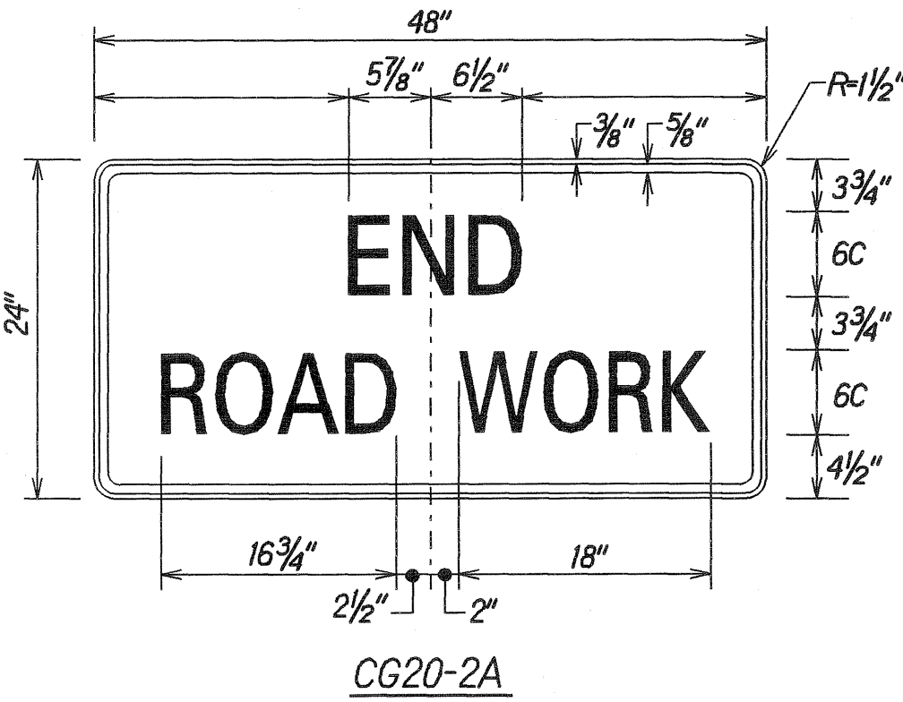
SIGN DETAILS Not To Scale
