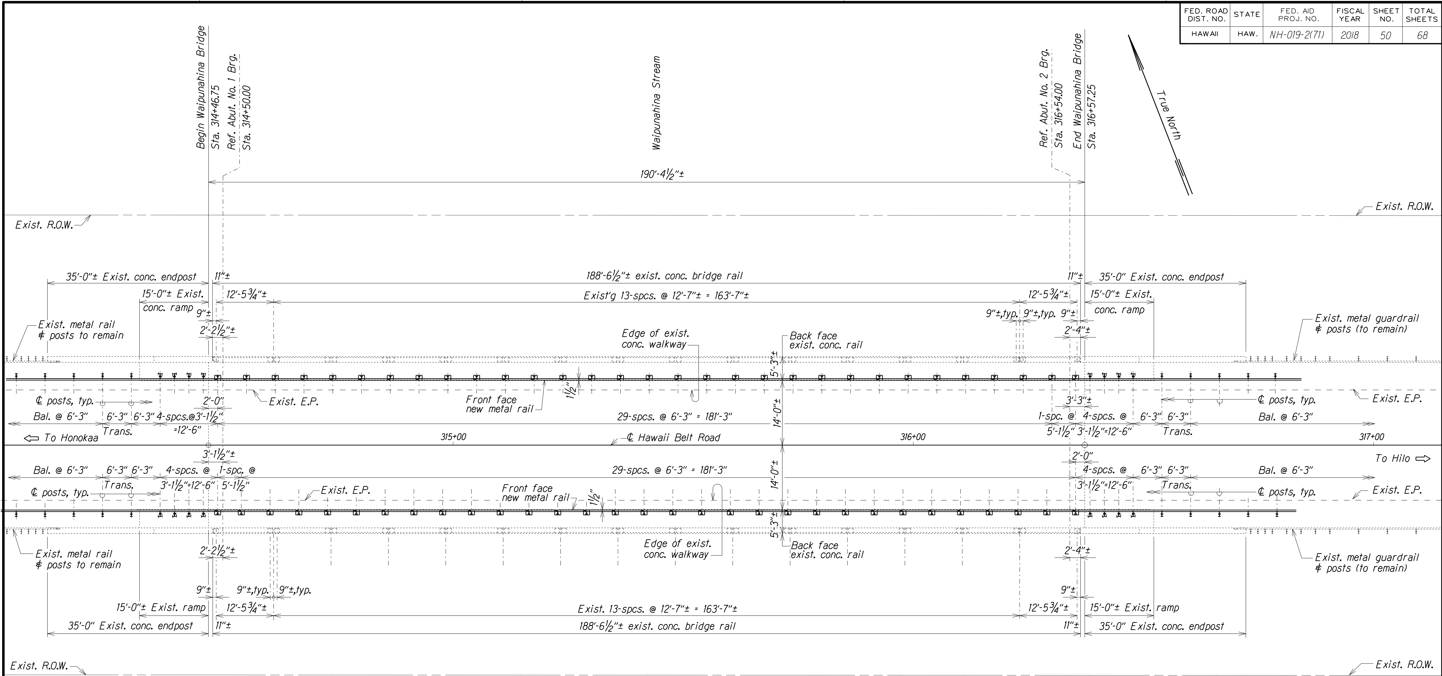
WAIPUNAHINA BRIDGE -- LAYOUT PLAN Scale: 1" = 10'
