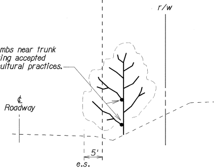
TRIMMING LATERAL BRANCHES OF TREES WITHIN THE STATE HIGHWAYS RIGHT-OF-WAY Pay Item 11.2 Scale: NONE
