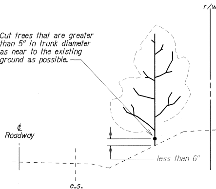
REMOVAL OF TREES Pay Item 11.3 Scale: NONE
