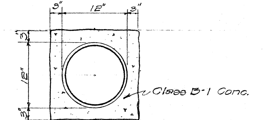
DETAIL OF CONCRETE JACKET Scale: 1" = 1'-0"
