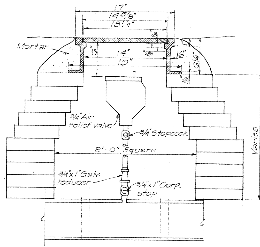
STANDARD BRICK VALVE BOX & AIR RELIEF VALVE ASSEMBLY Scale: 1/2" = 1'-0"
