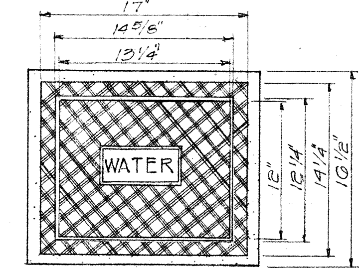
STANDARD C.I. FRAME & COVER
