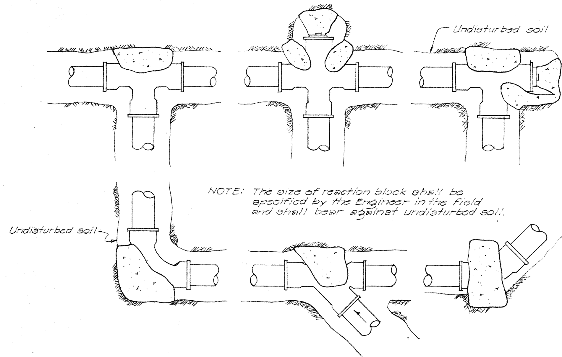
CONCRETE REACTION BLOCKS FOR WATER MAINS
