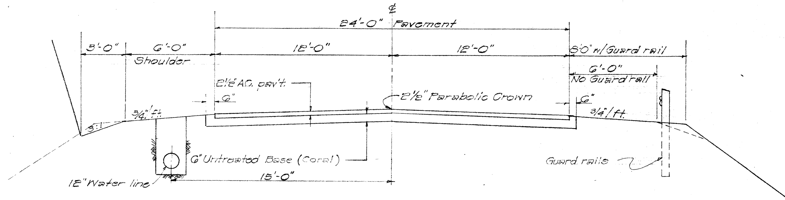
TYPICAL ROAD SECTION WITH PIPELINE Scale: 1/4" = 1'-0"
