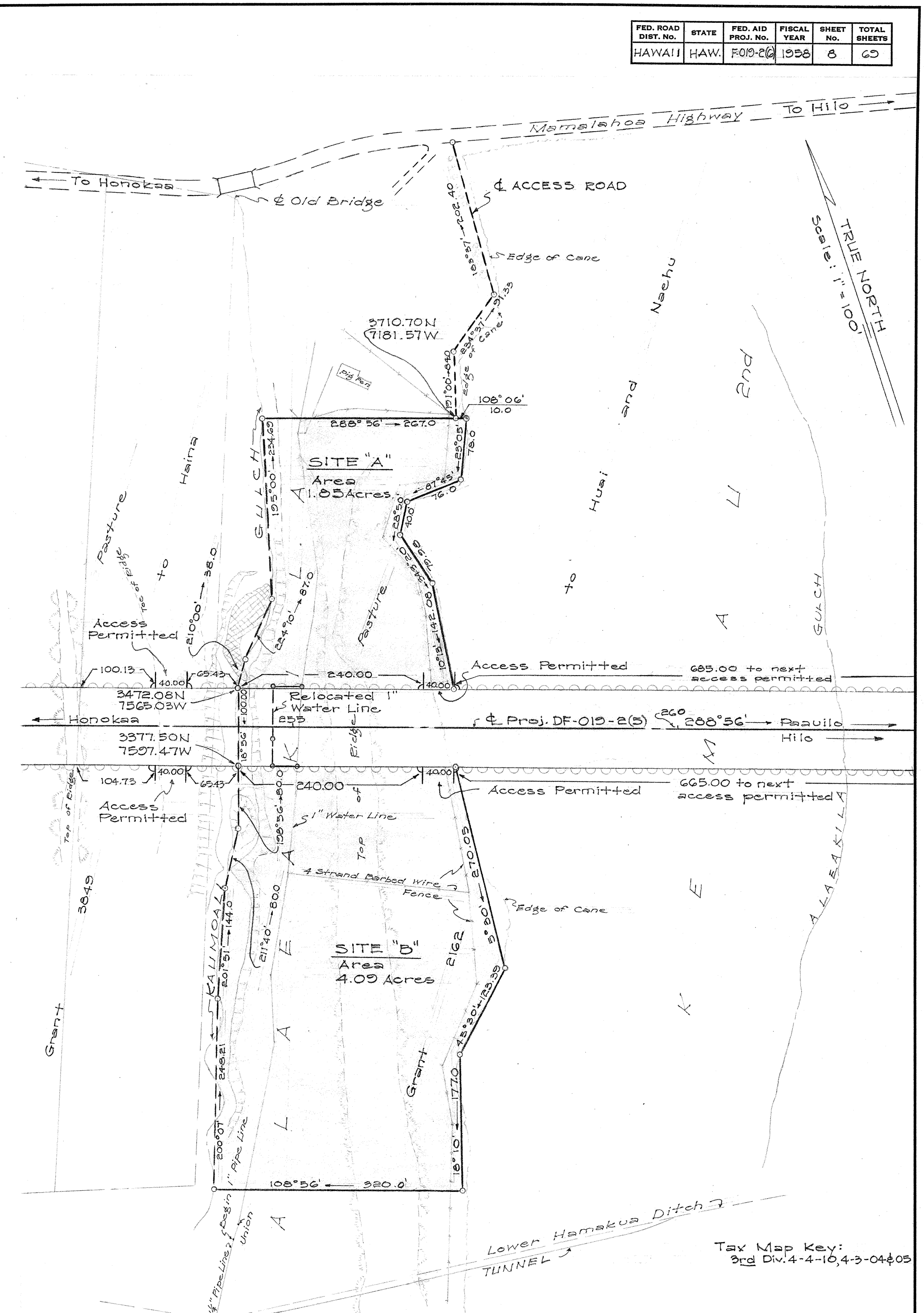
PROPOSED BORROW PIT SITES Scale: 1"=100'
