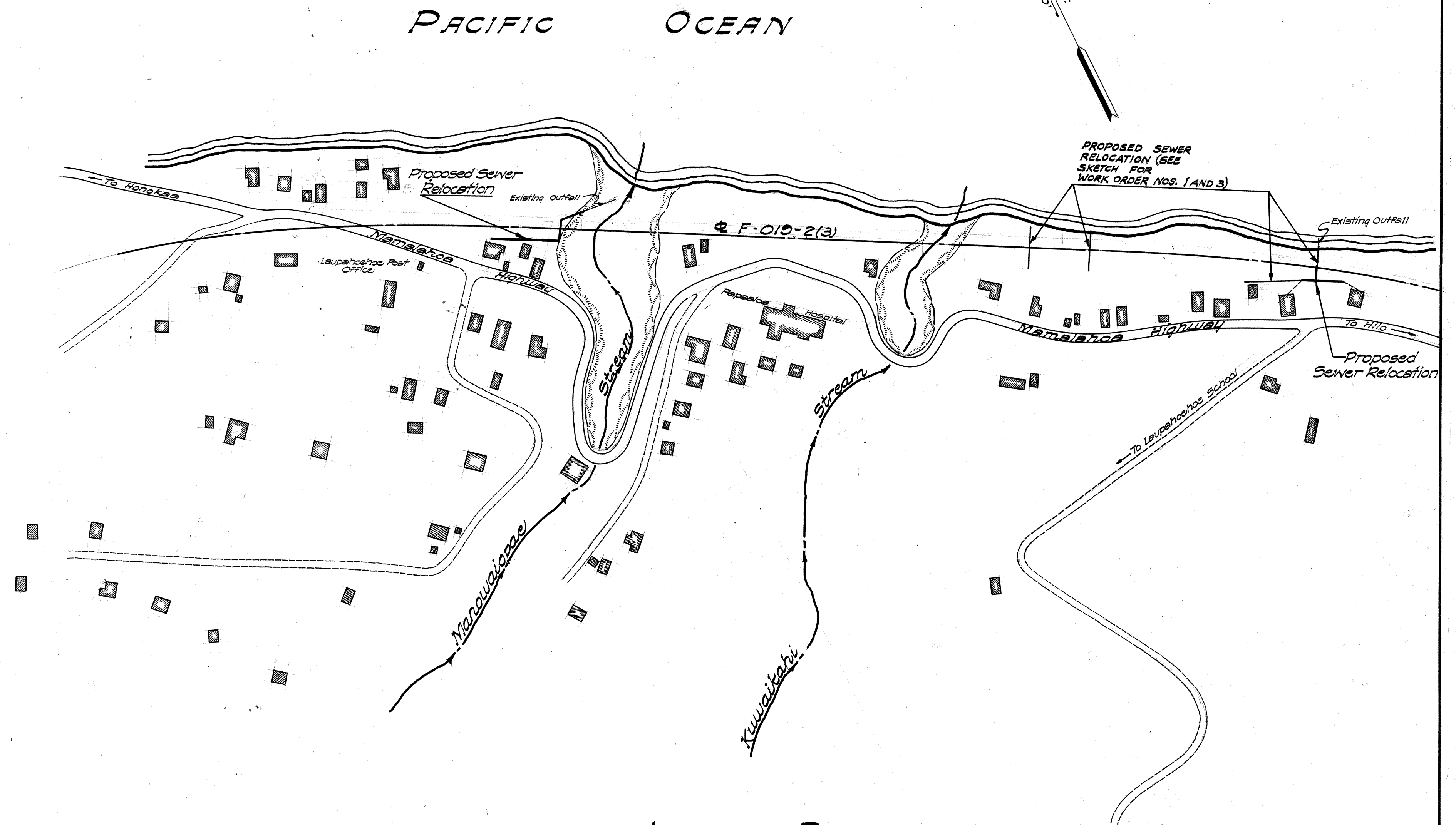
LOCATION PLAN LAUPAHOEHOE Scale 1 in.=200 Ft.
