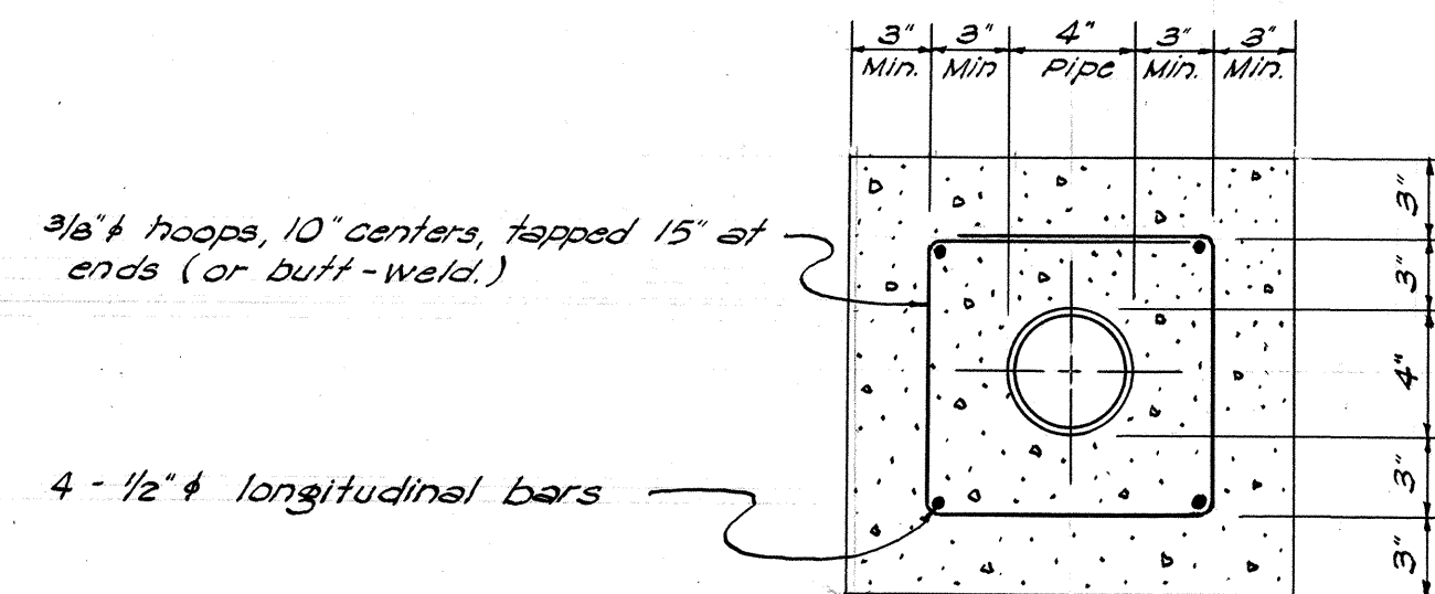
DETAIL OF SEWER JACKET Scale: 1/2"=1'0"
