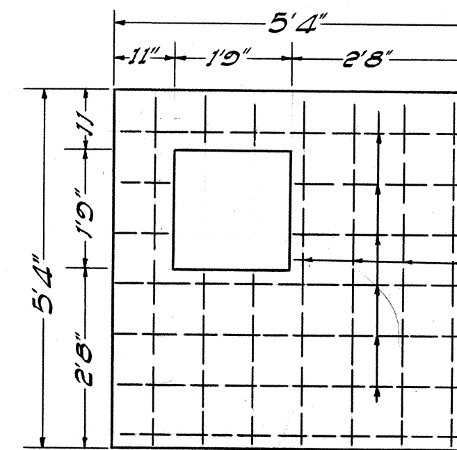
TOP SLAB REINFORCING
