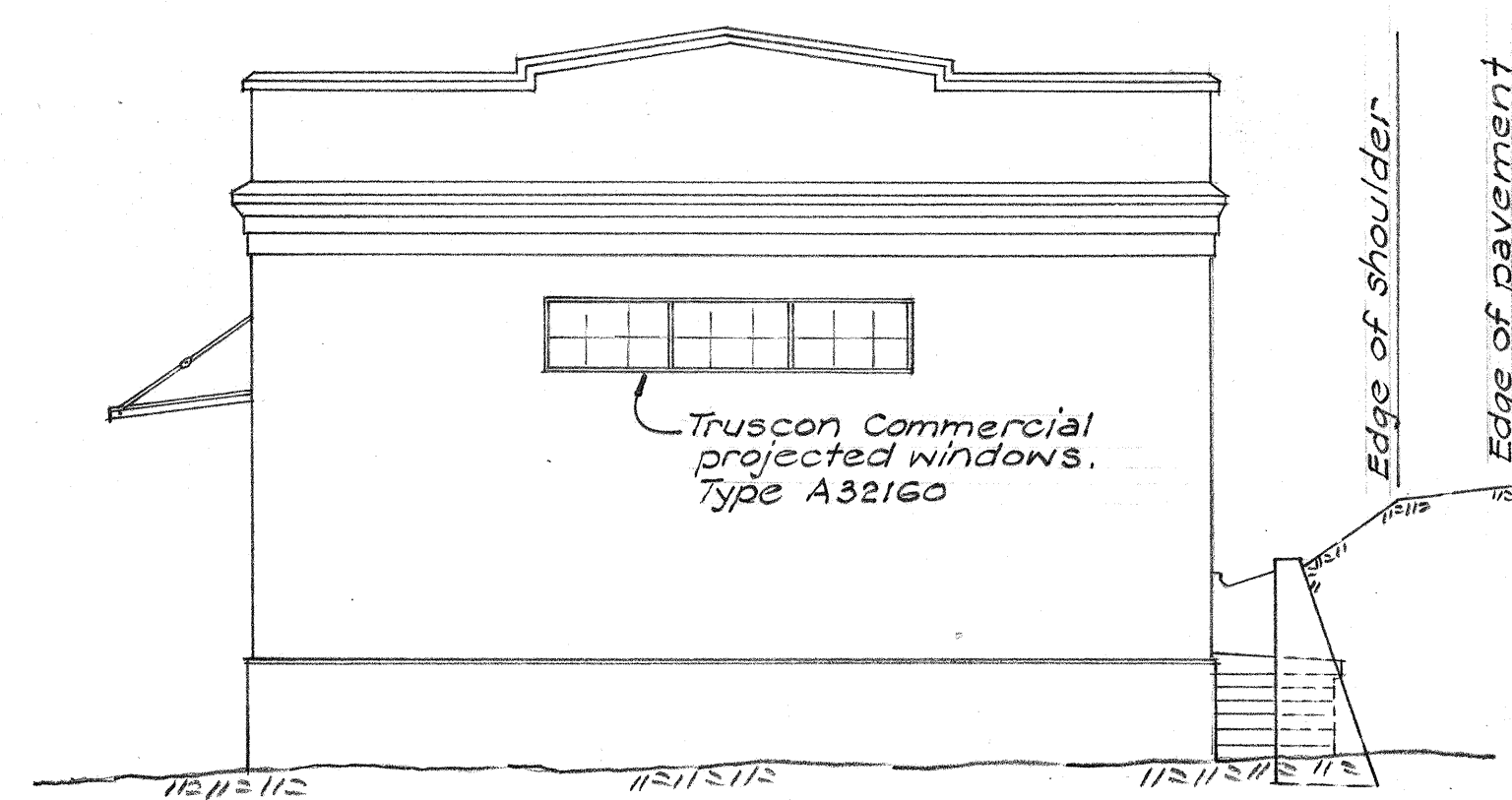
END ELEVATION SHOWING NEW WINDOW 3" = 1'-0"
