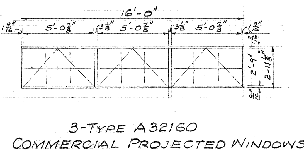
WINDOW DETAIL 3" = 1'-0"
