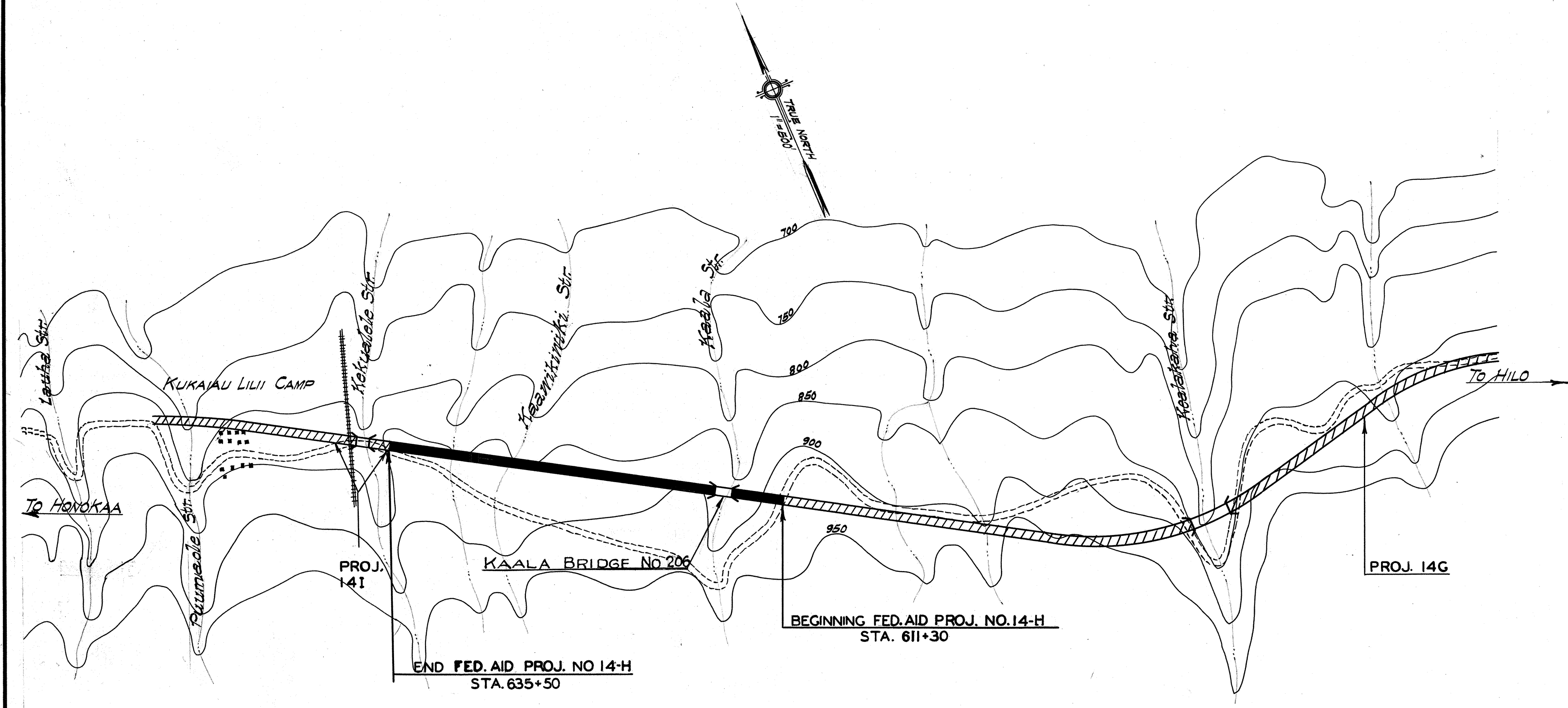
LAYOUT OF PROJECT Scale 1"=500'
