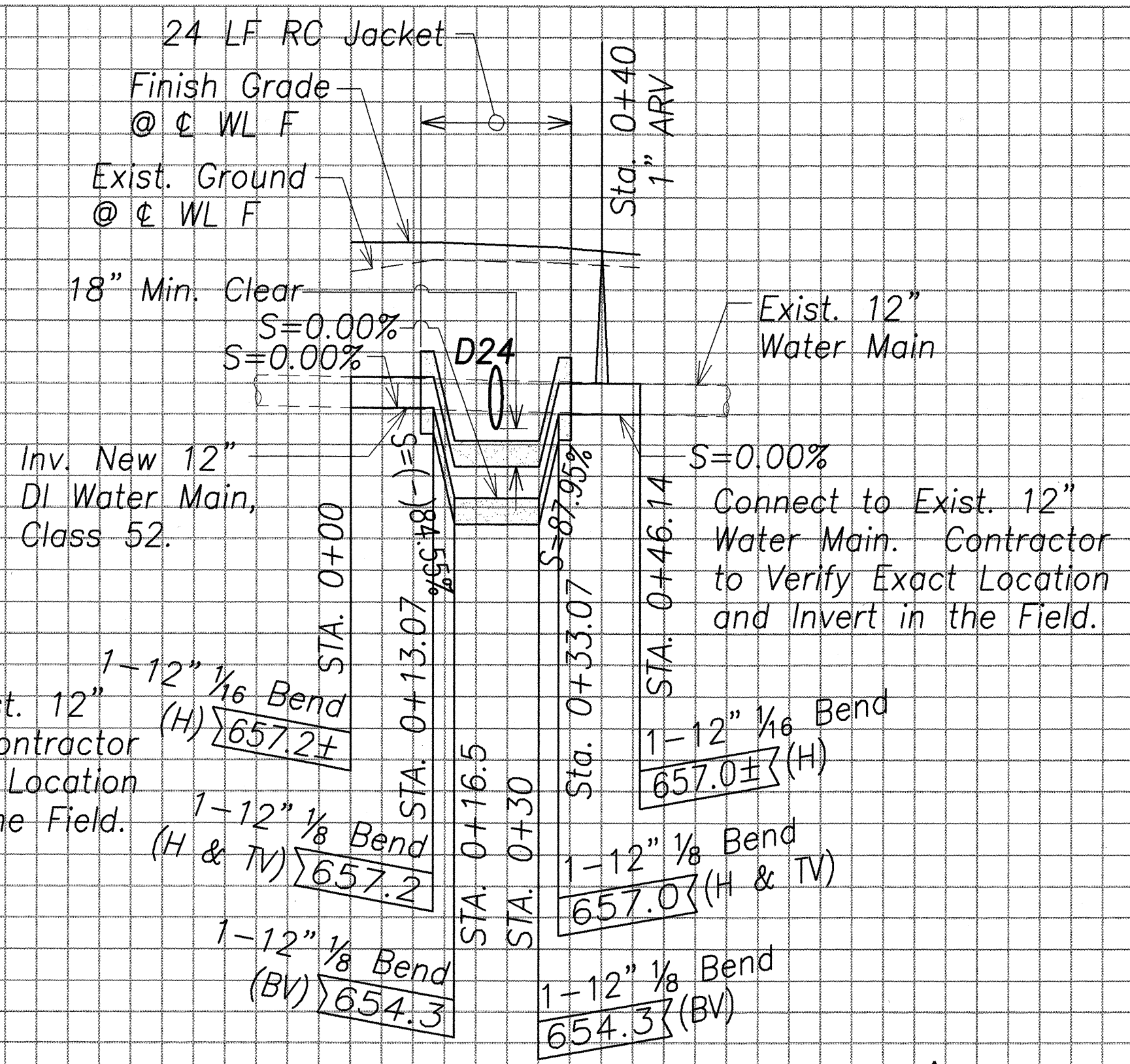
PROFILE - WATER LINE B
