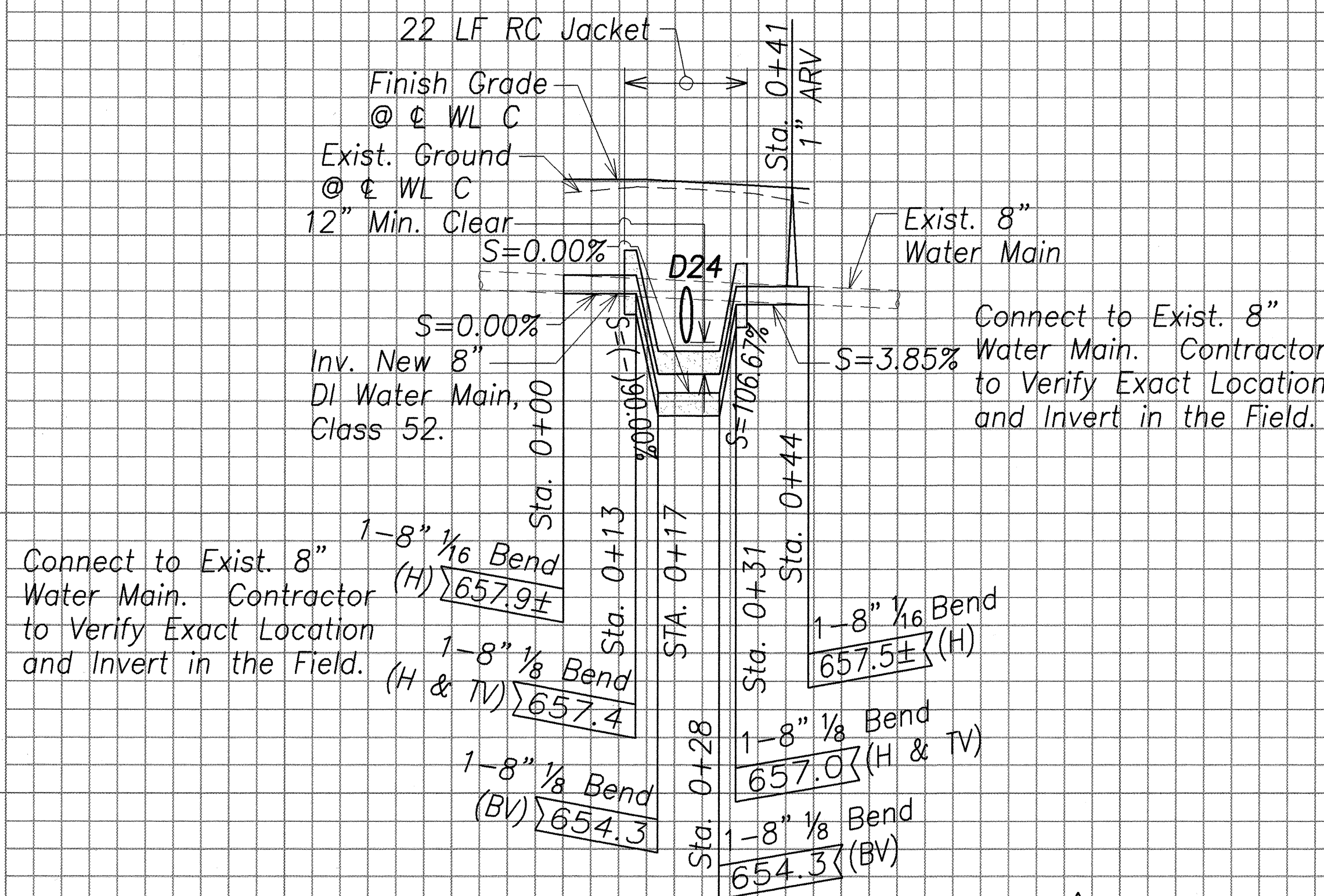
PROFILE - WATER LINE A
