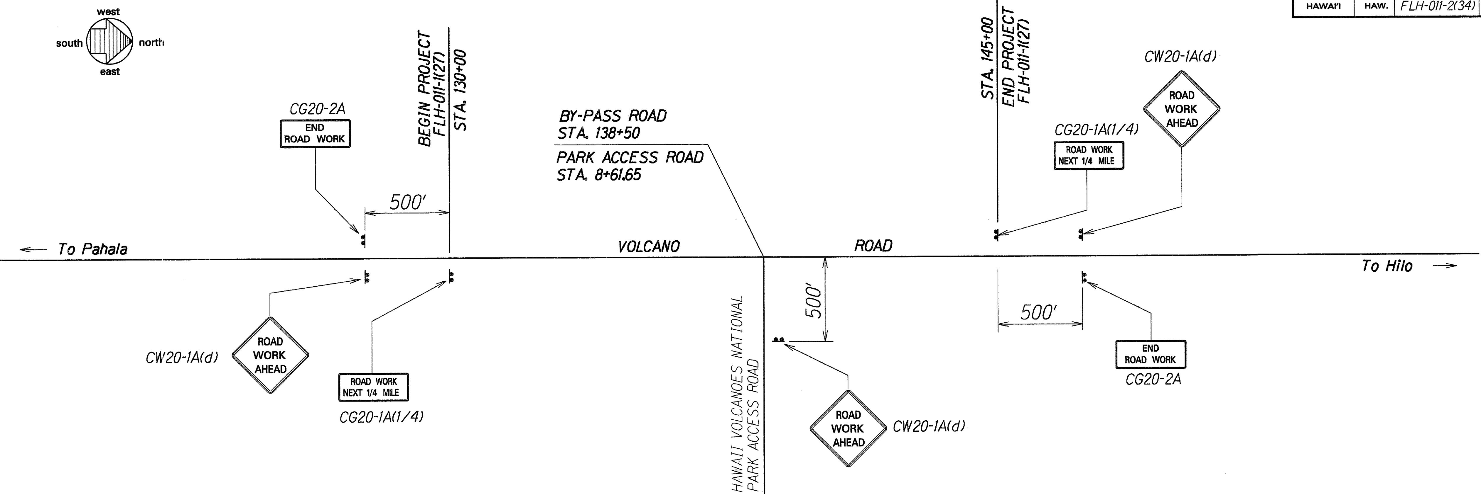
CONSTRUCTION SIGN PLAN Not To Scale
