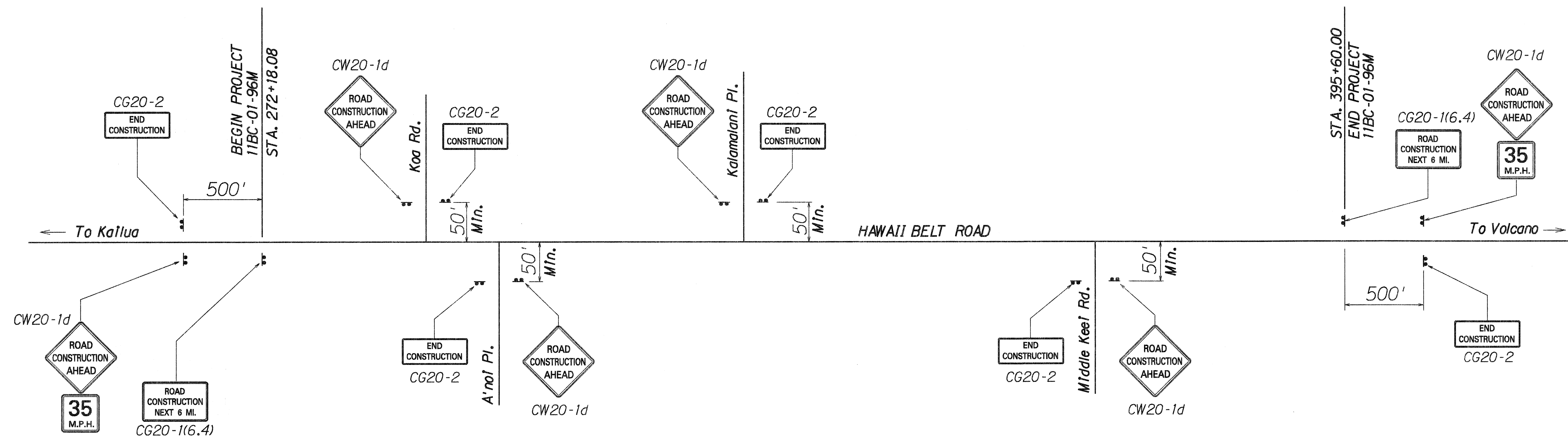
CONSTRUCTION SIGN PLAN Not To Scale
