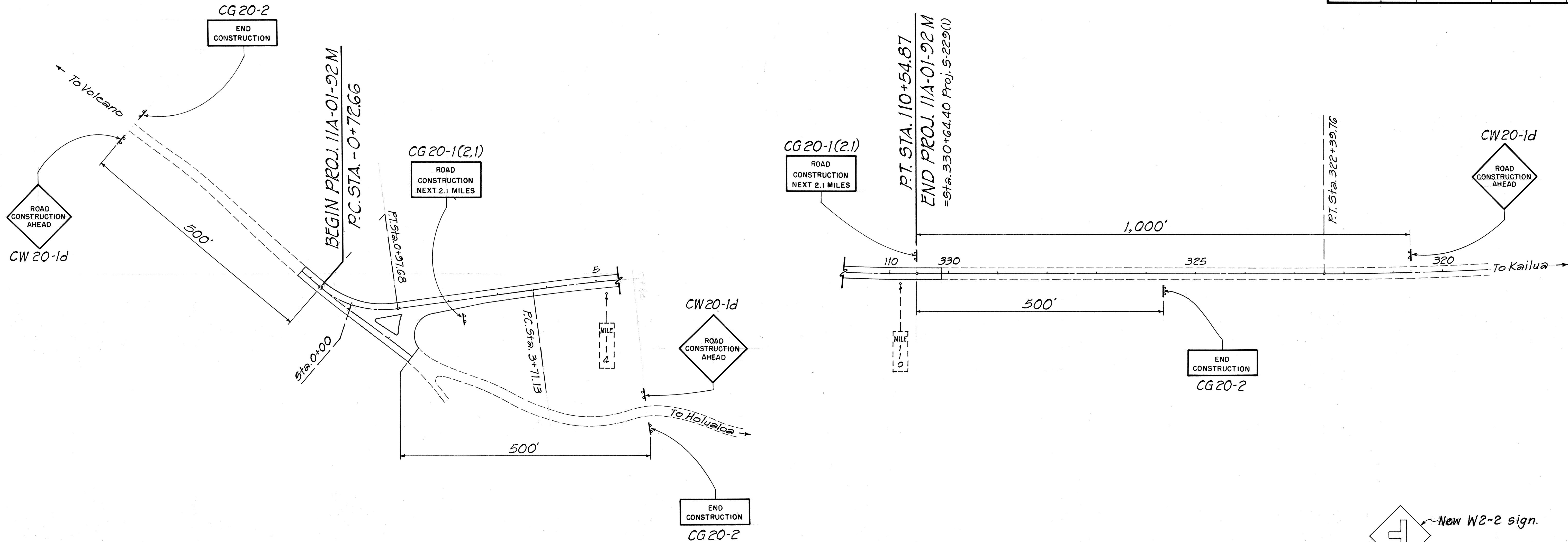
CONSTRUCTION SIGN DETAIL Not To Scale
