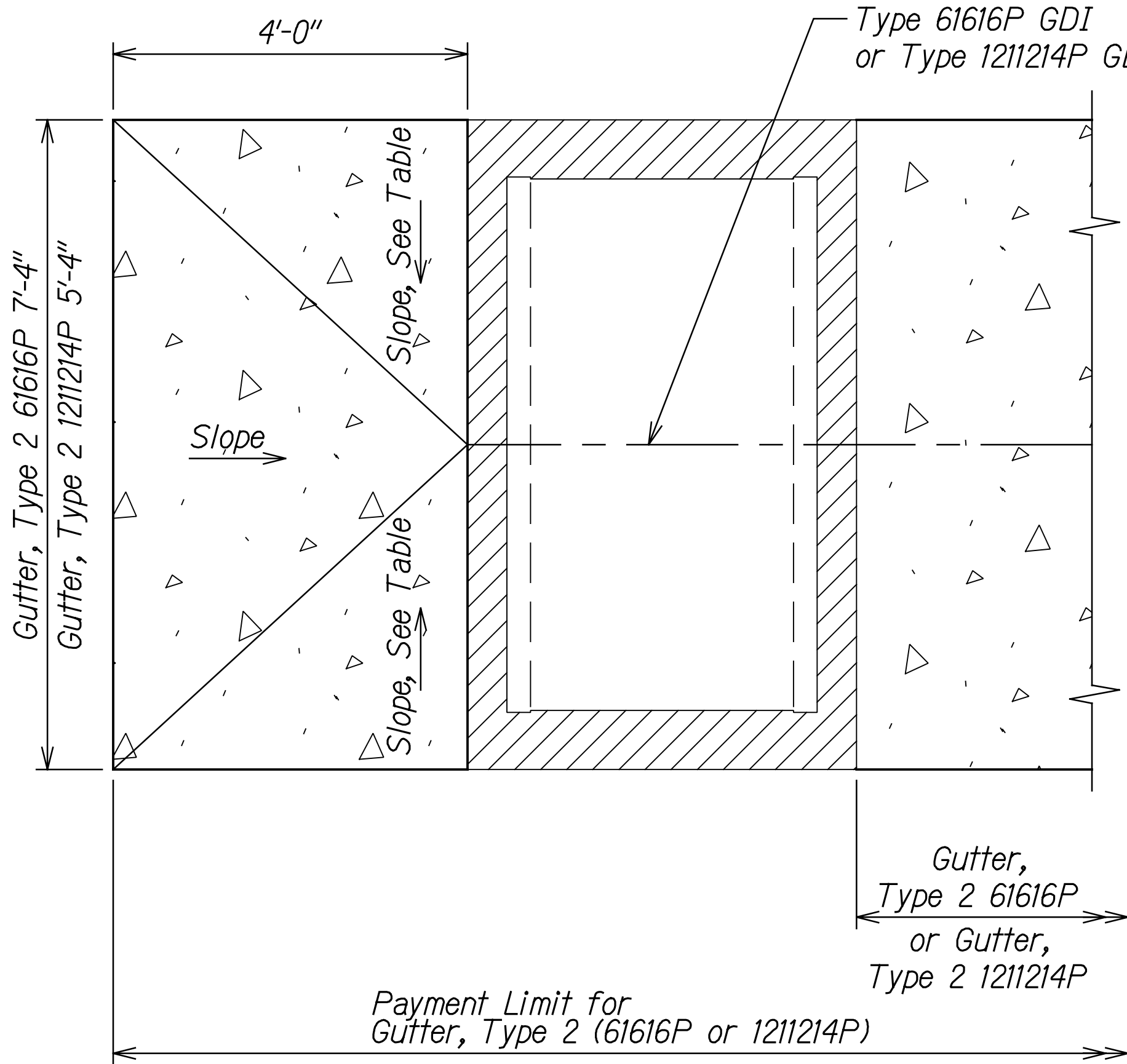
BEGIN AND END OF GUTTER DETAIL Not to Scale
