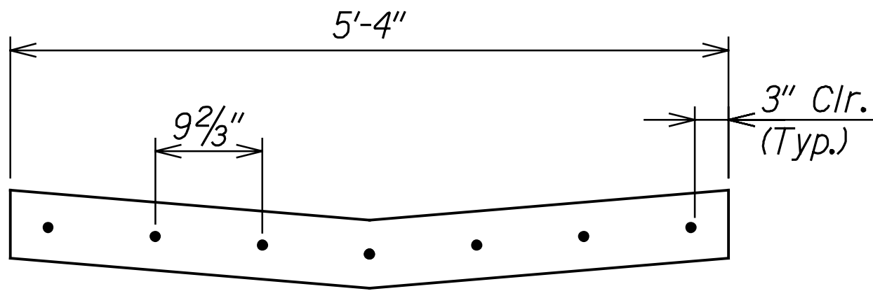
GUTTER, TYPE 2 1211214P DOWEL PLACEMENT AT JOINT LOCATIONS Scale 1" = 1'-0"
