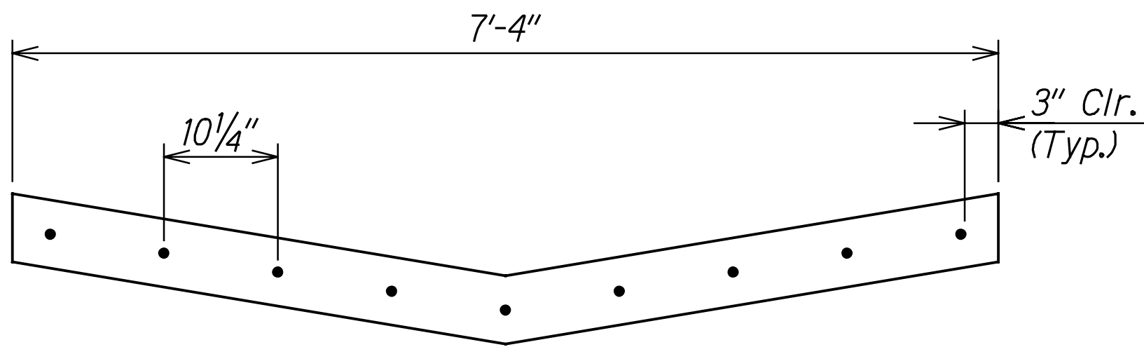
GUTTER, TYPE 2 61616P DOWEL PLACEMENT AT JOINT LOCATIONS Scale 1" = 1'-0"
