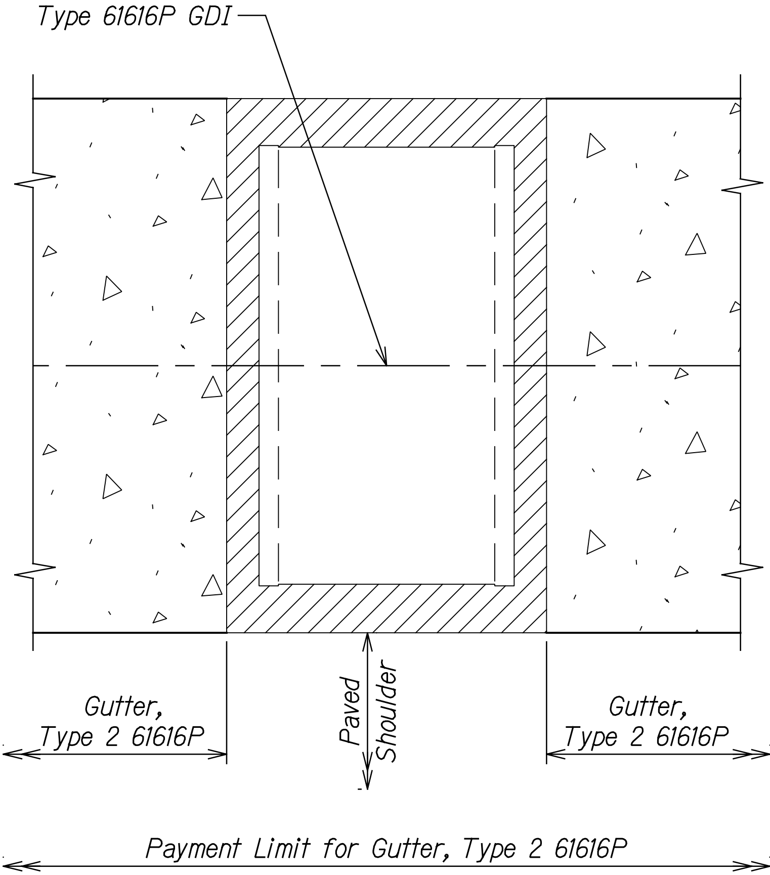
GUTTER AT GDI DETAIL Not to Scale
