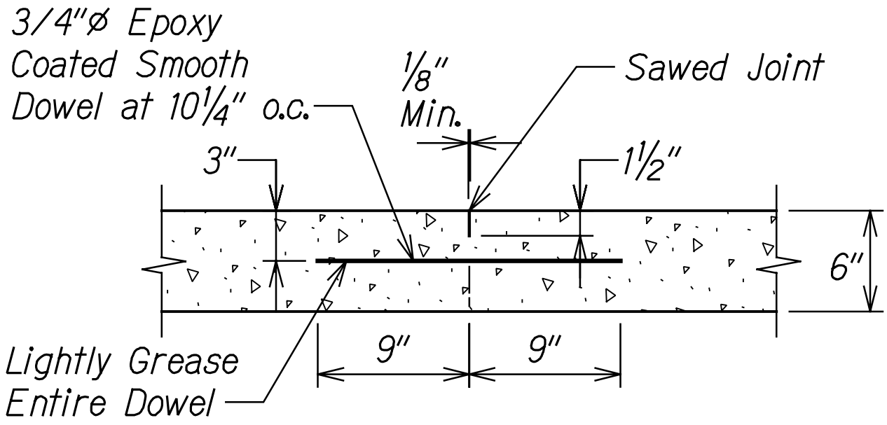
CONTRACTION JOINT DETAIL Not to Scale
