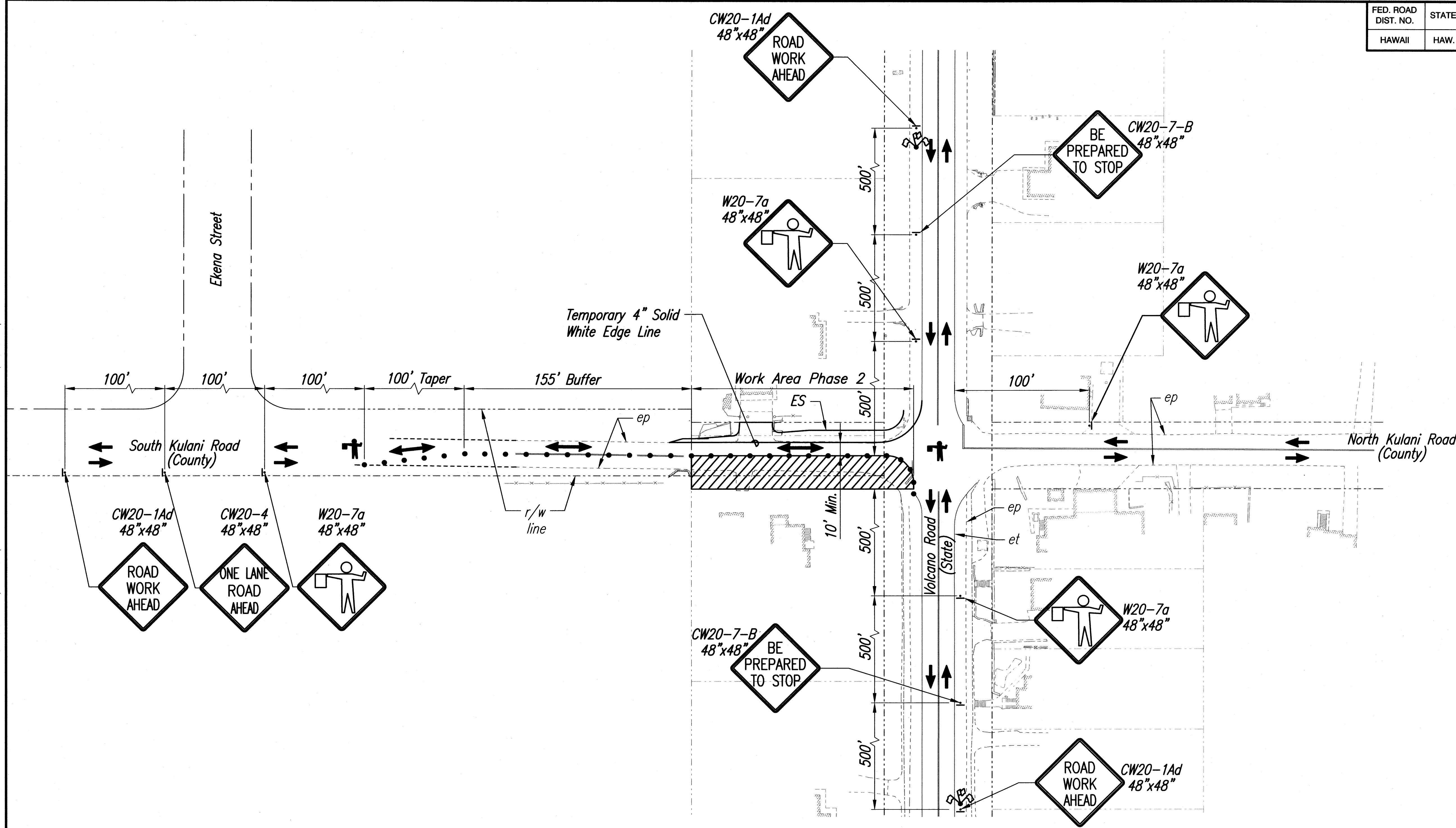
TRAFFIC CONTROL PHASE - 2 SCALE: 1"=40'
