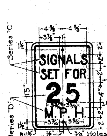
R-10 12" x 18"
