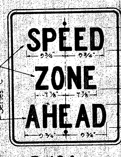
R-104 24" x 30"
