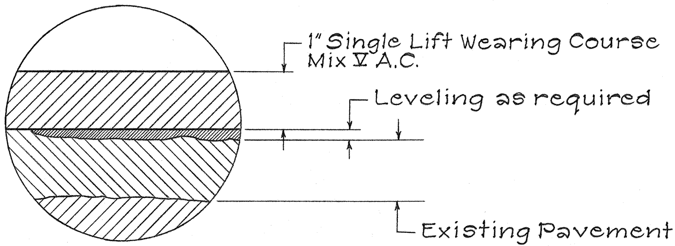
PAVEMENT DETAIL NOT TO SCALE
