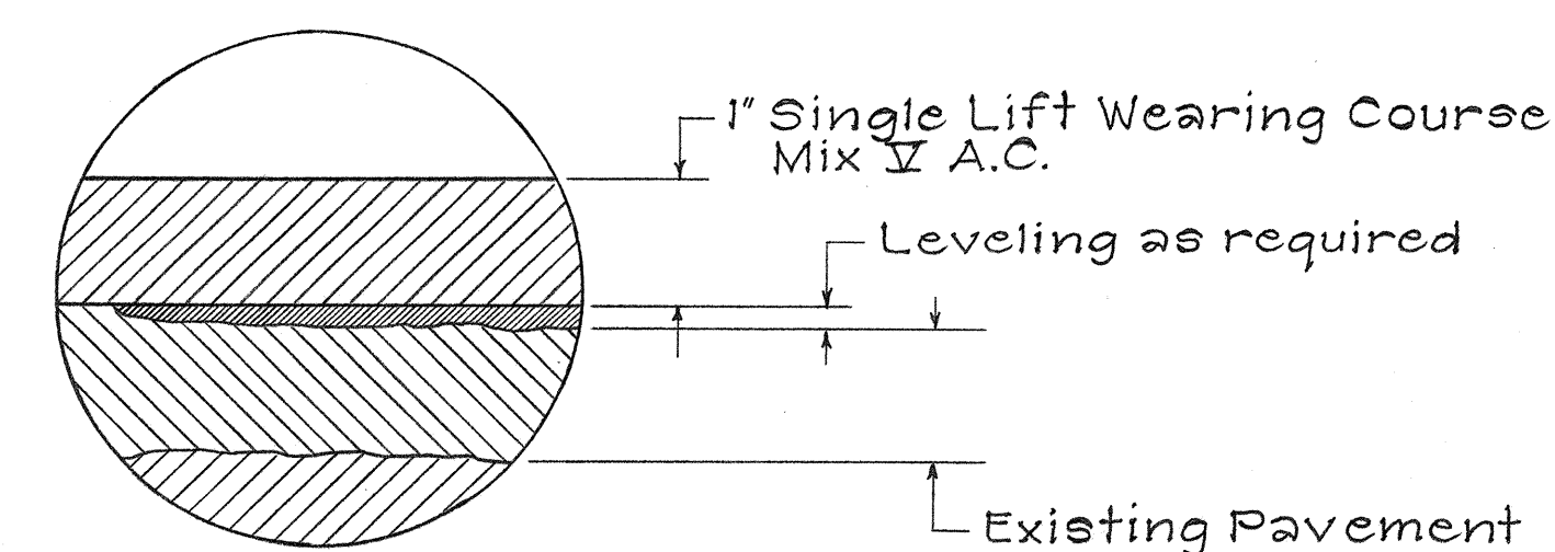
PAVEMENT DETAIL NOT TO SCALE
