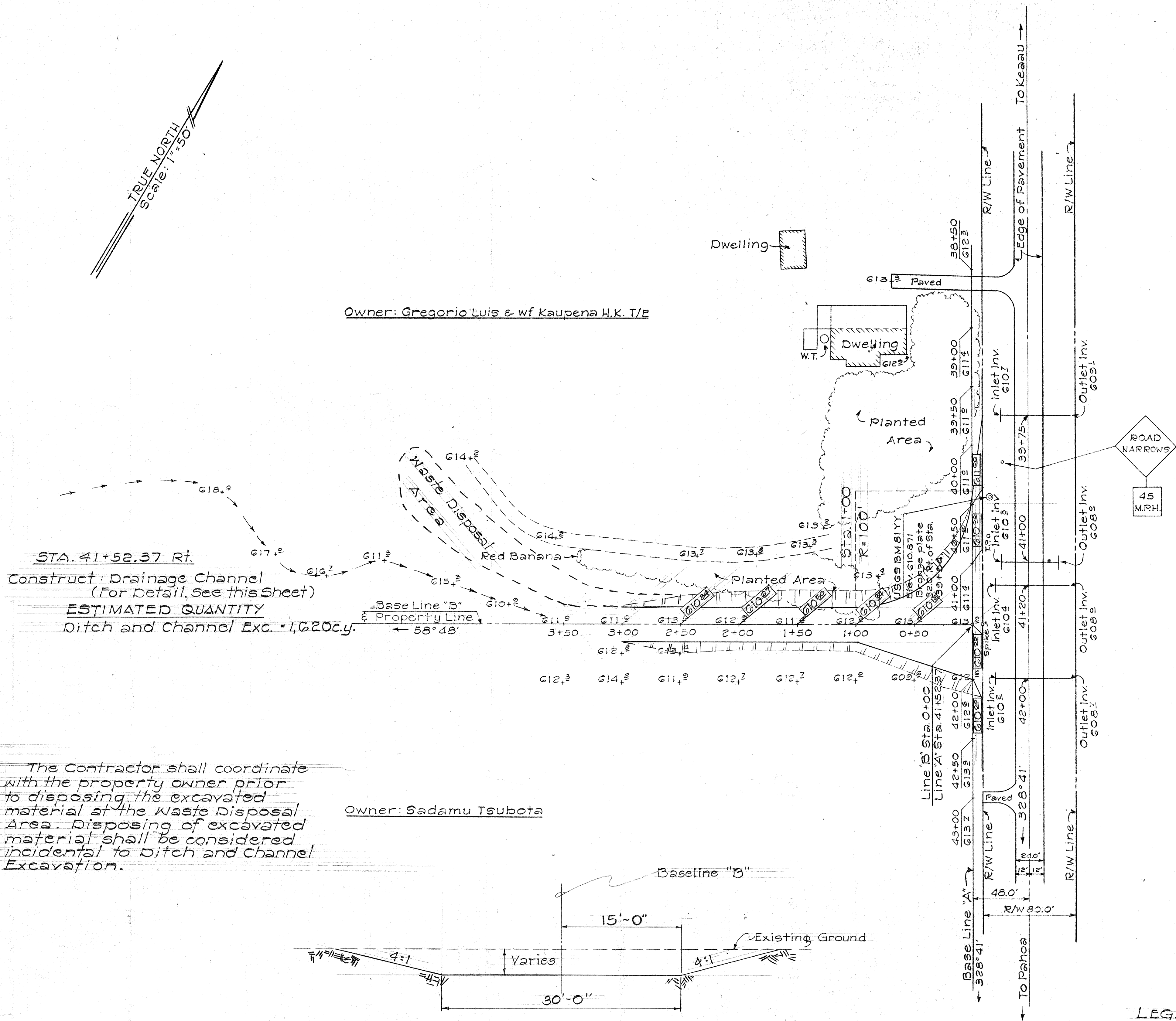
TYPICAL SECTION Not to Scale
