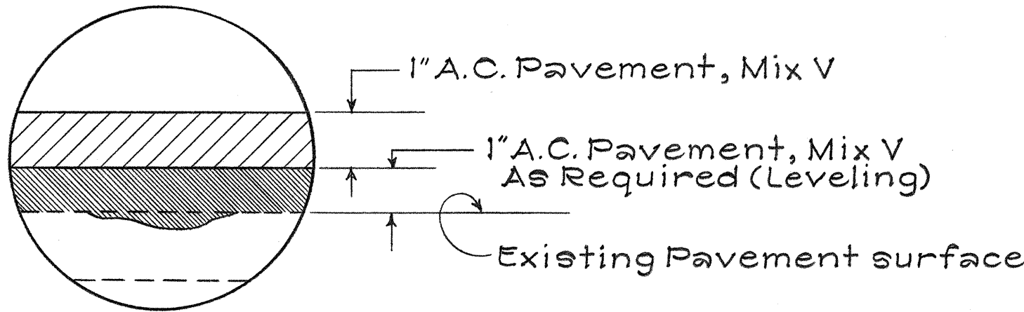
PAVEMENT DETAIL Not to Scale
