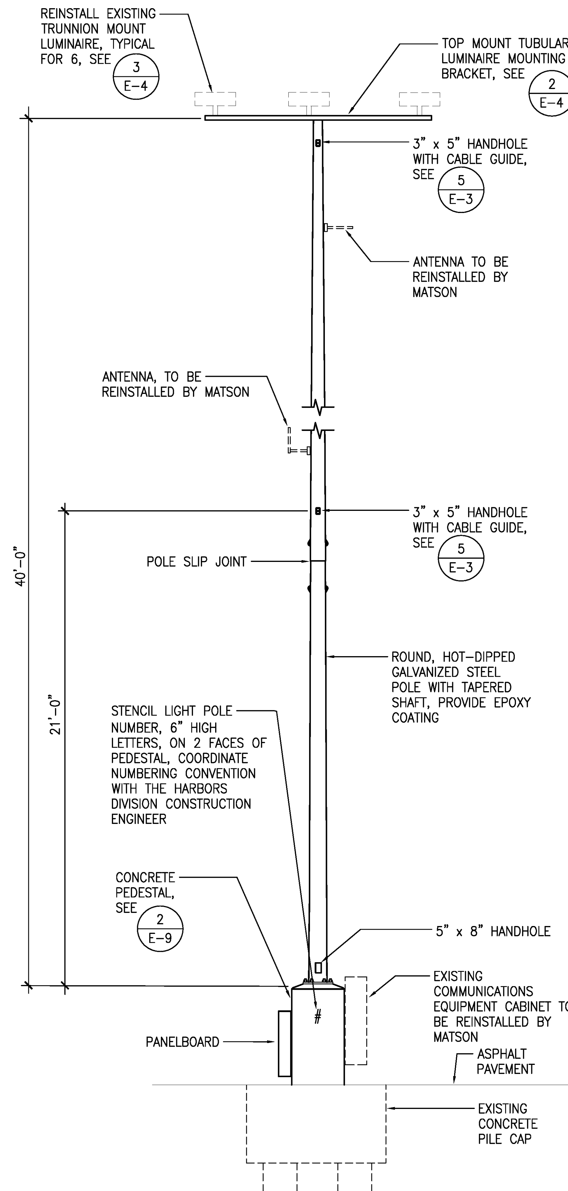
2 NEW LIGHT POLE DETAIL (POLE 36) E-5 NOT TO SCALE
