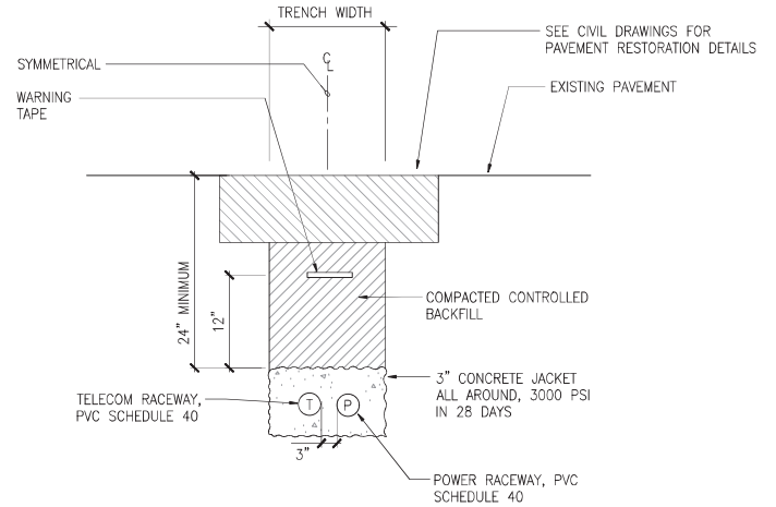
2 TYPICAL TELECOM AND POWER CONCRETE ENCASED DUCT SECTION E-2 NOT TO SCALE
