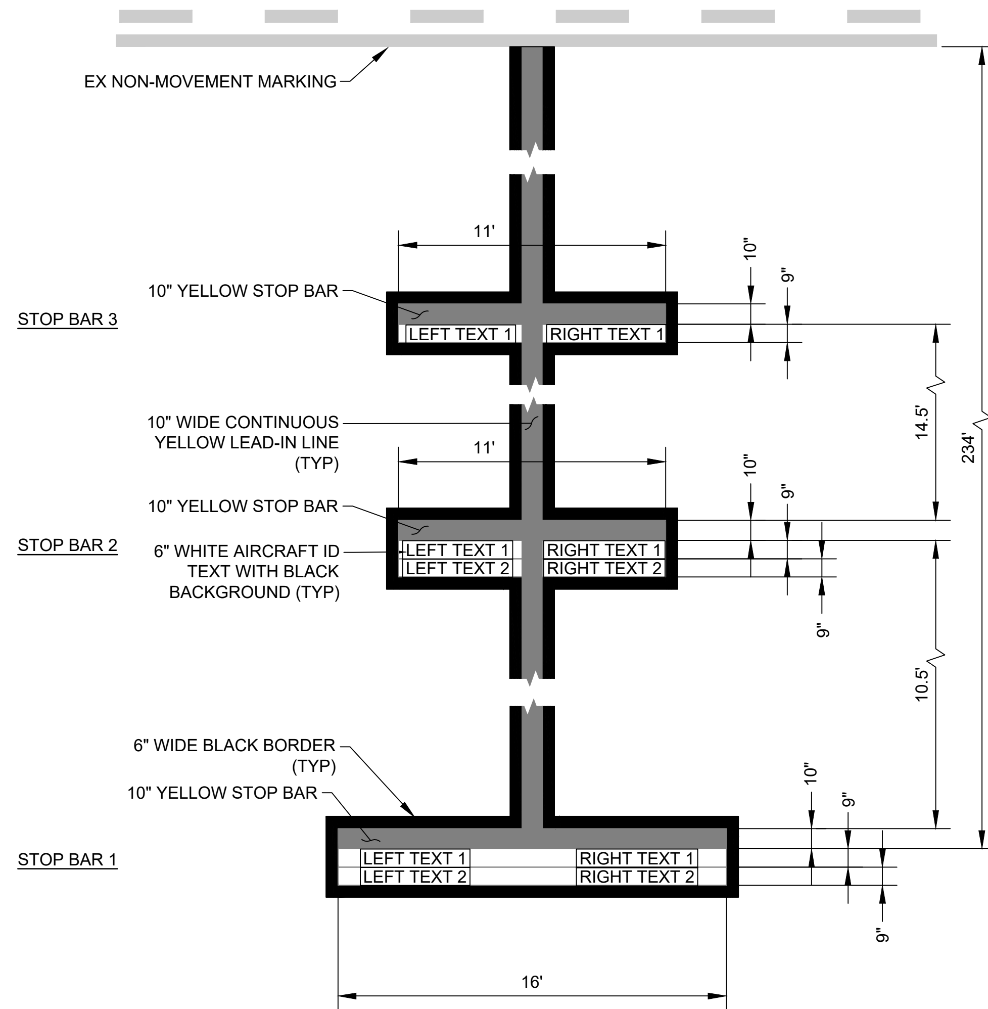
7 SPOT 8 LEAD-IN LINE AND STOP BAR MARKINGS C-107 C-108 SCALE: NTS
