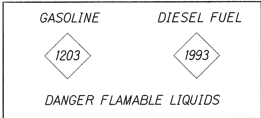
END VIEW GASOLINE/DIESEL TANK Not to Scale
