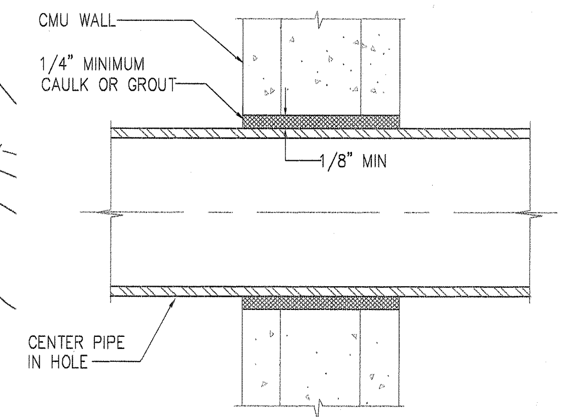
PIPE THRU INTERIOR CMU WALL DETAIL NOT TO SCALE
