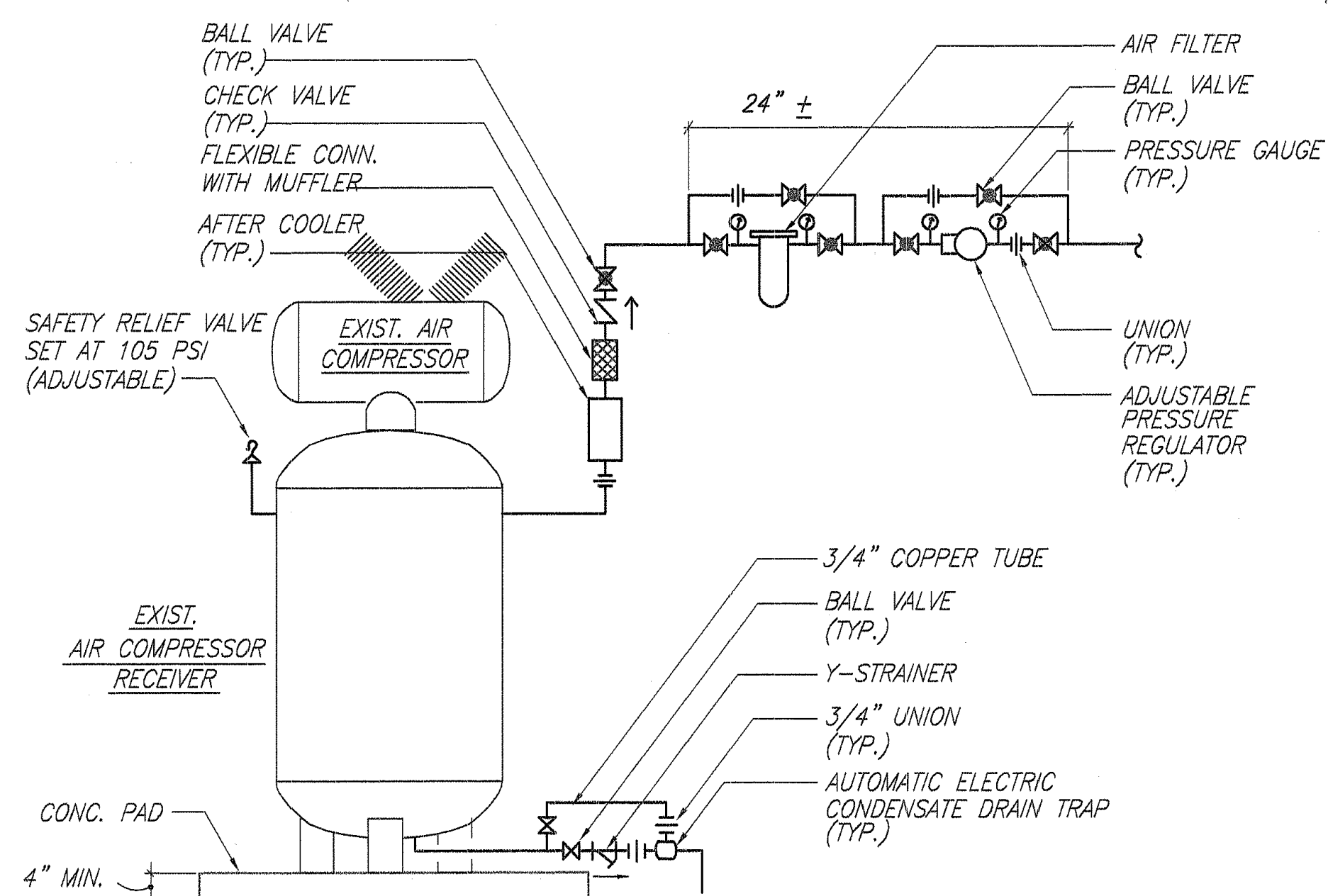
AIR COMPRESSOR PIPING SCHEMATIC NOT TO SCALE
