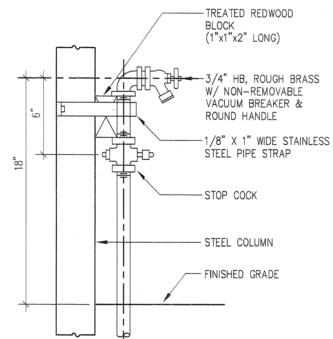
HOSE BIBB-INTERIOR NOT TO SCALE
