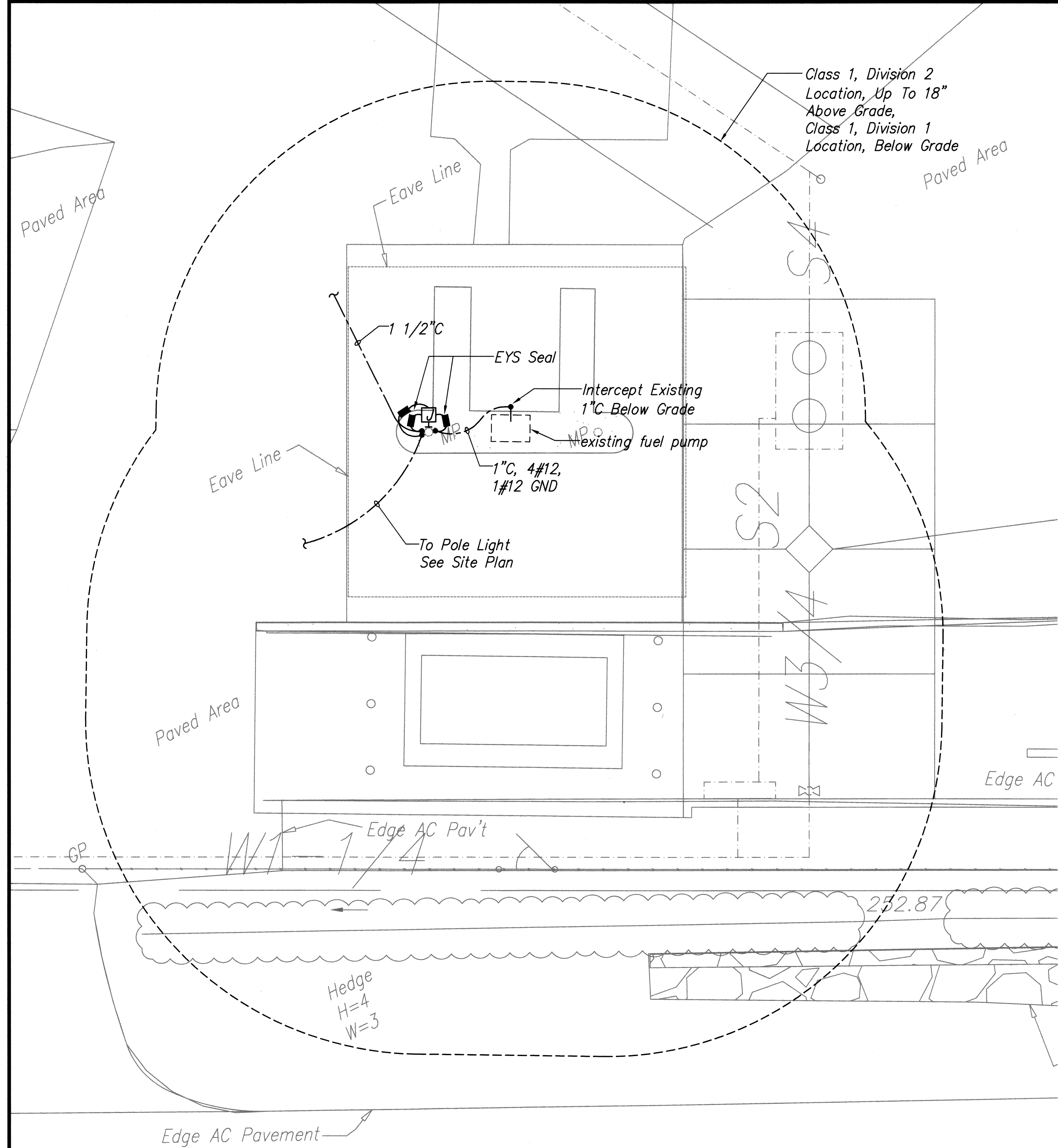
FUEL DISPENSER POWER PLAN Scale: 1/4" = 1'-0" E-6 | 1 | E-6
