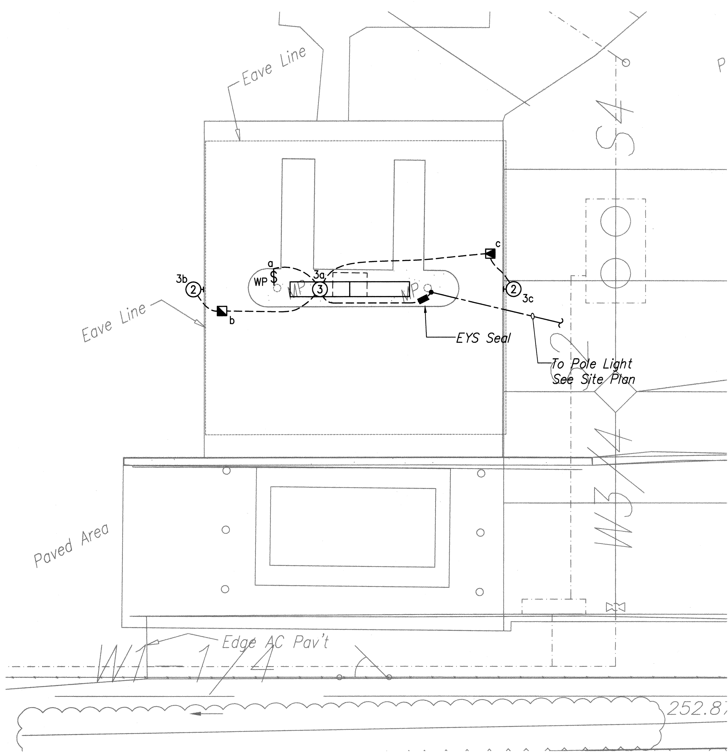
FUEL DISPENSER LIGHTING PLAN Scale: 1/4" = 1'-0" E-6 | 2 | E-6
