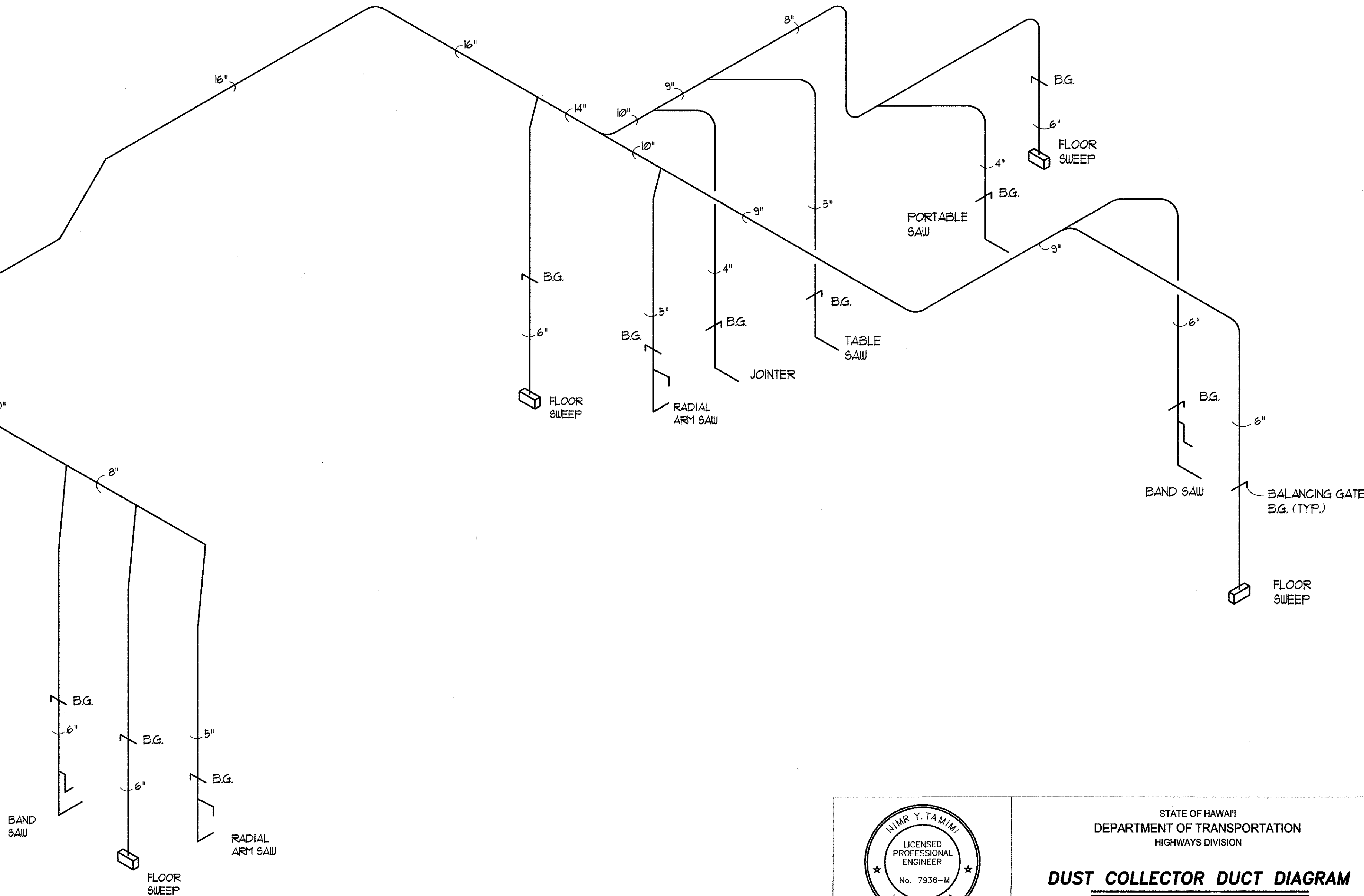
DUST COLLECTOR DUCT DIAGRAM NOT TO SCALE
