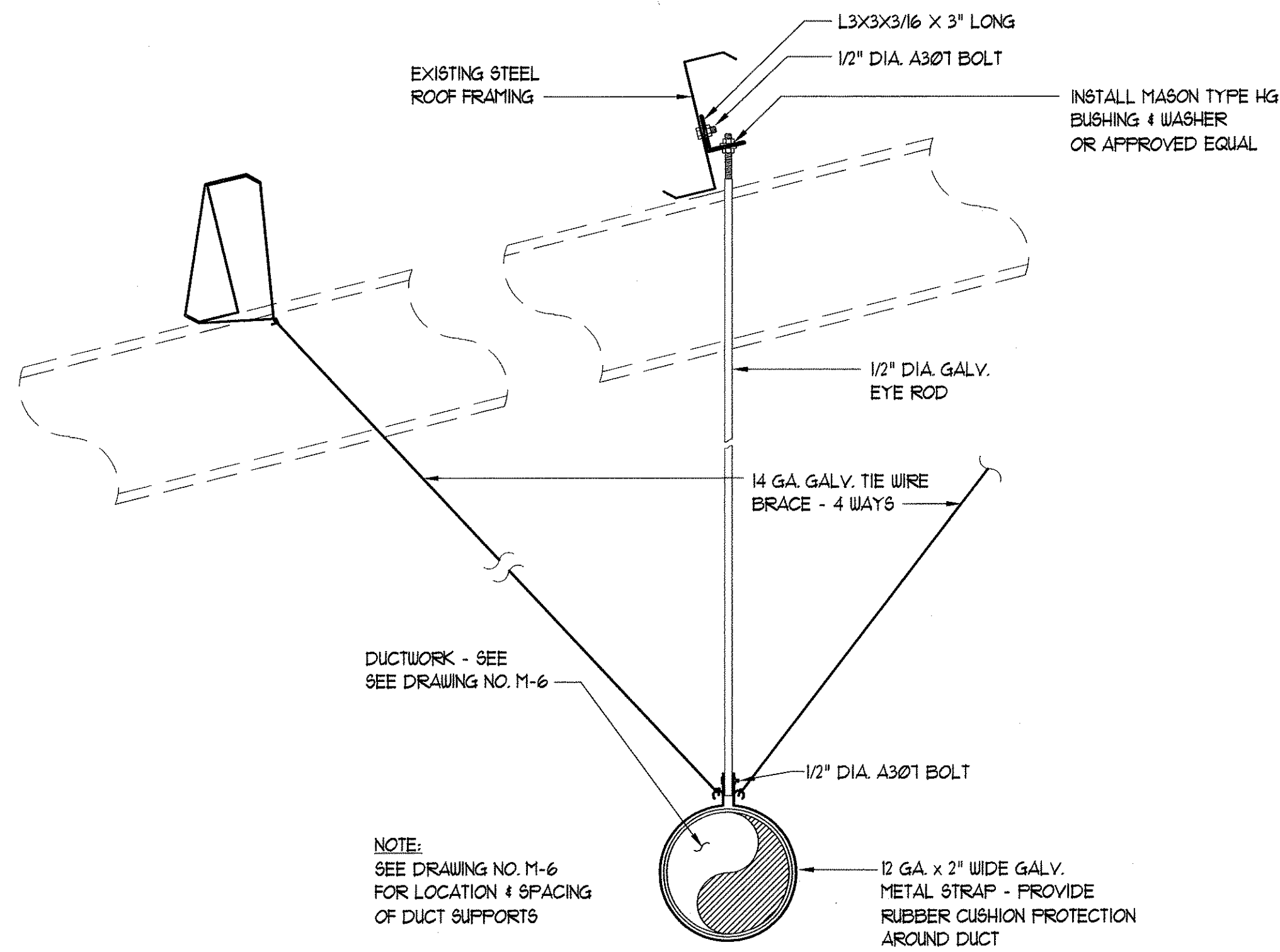
TYP. OVERHEAD DUCT SUPPORT M-11 NOT TO SCALE
